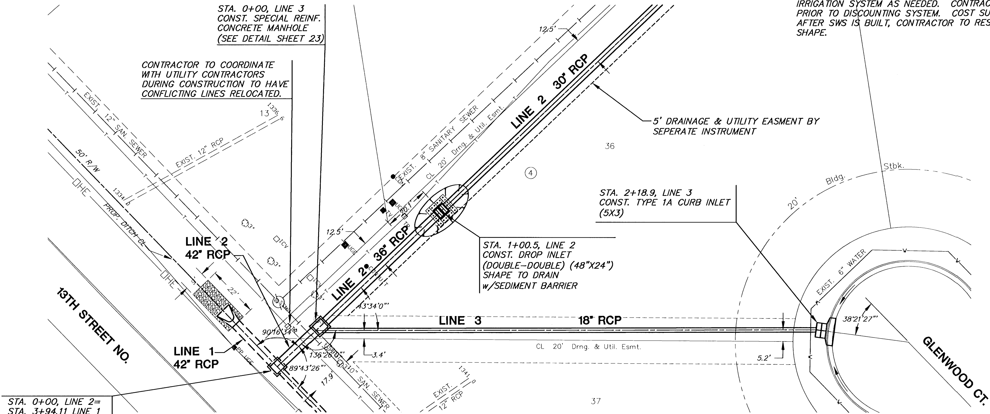
PLAN LINES 3 AND 2
