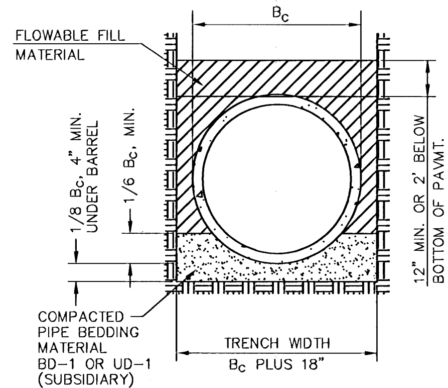
DETAIL OF FLOWABLE FILL FOR STORM SEWER PIPE EXCEPT CORRUGATED METAL PIPE.
