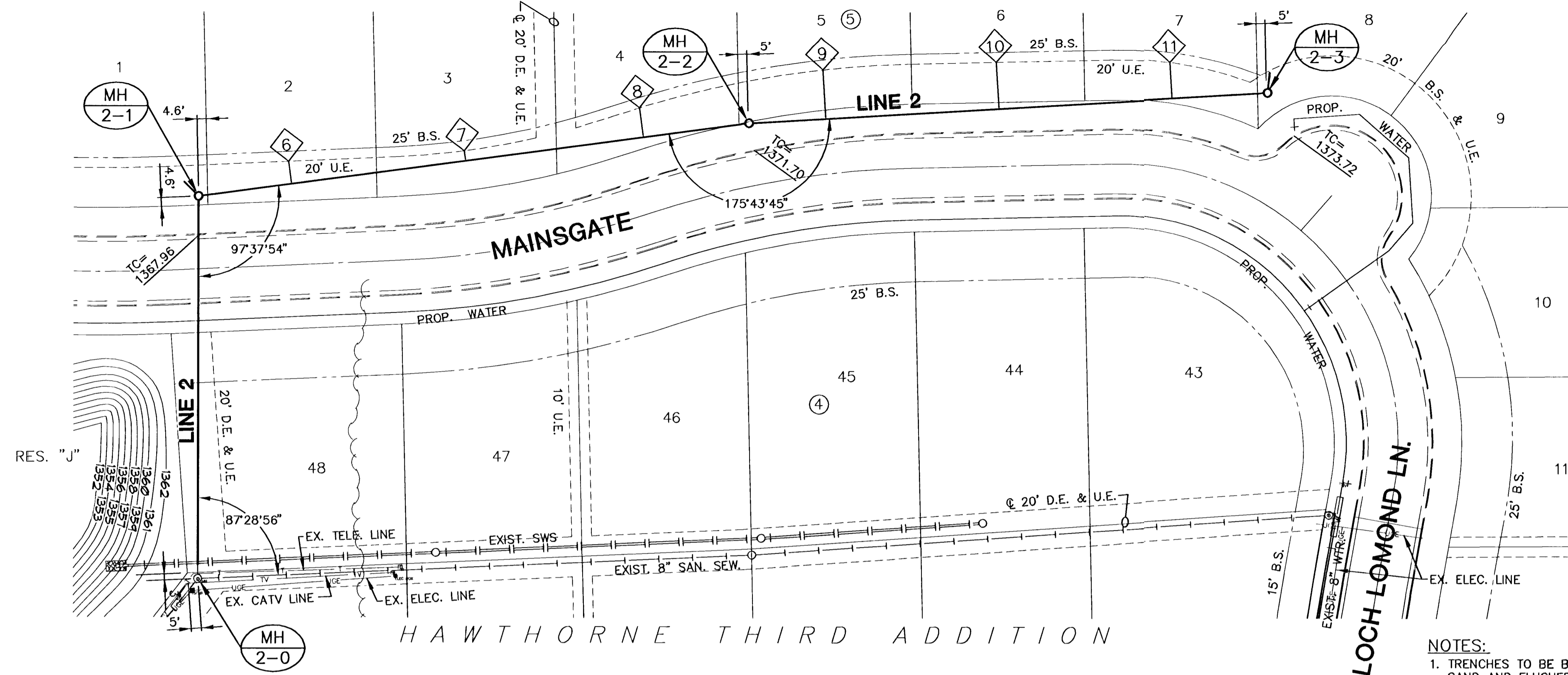
PLAN LINE 2
