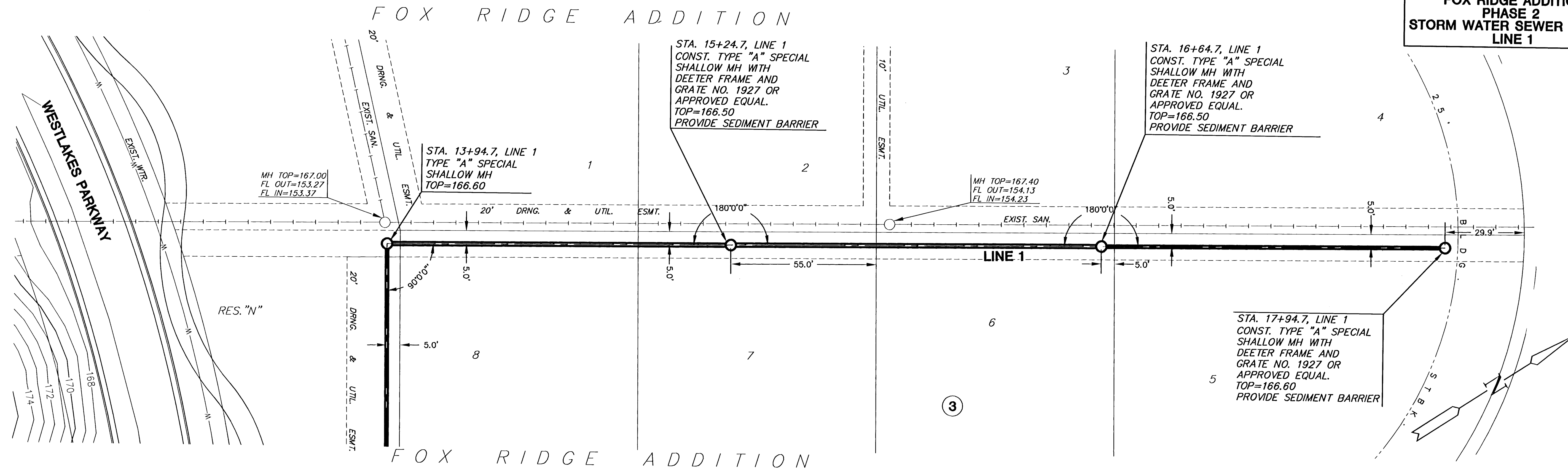
PLAN LINE 1
