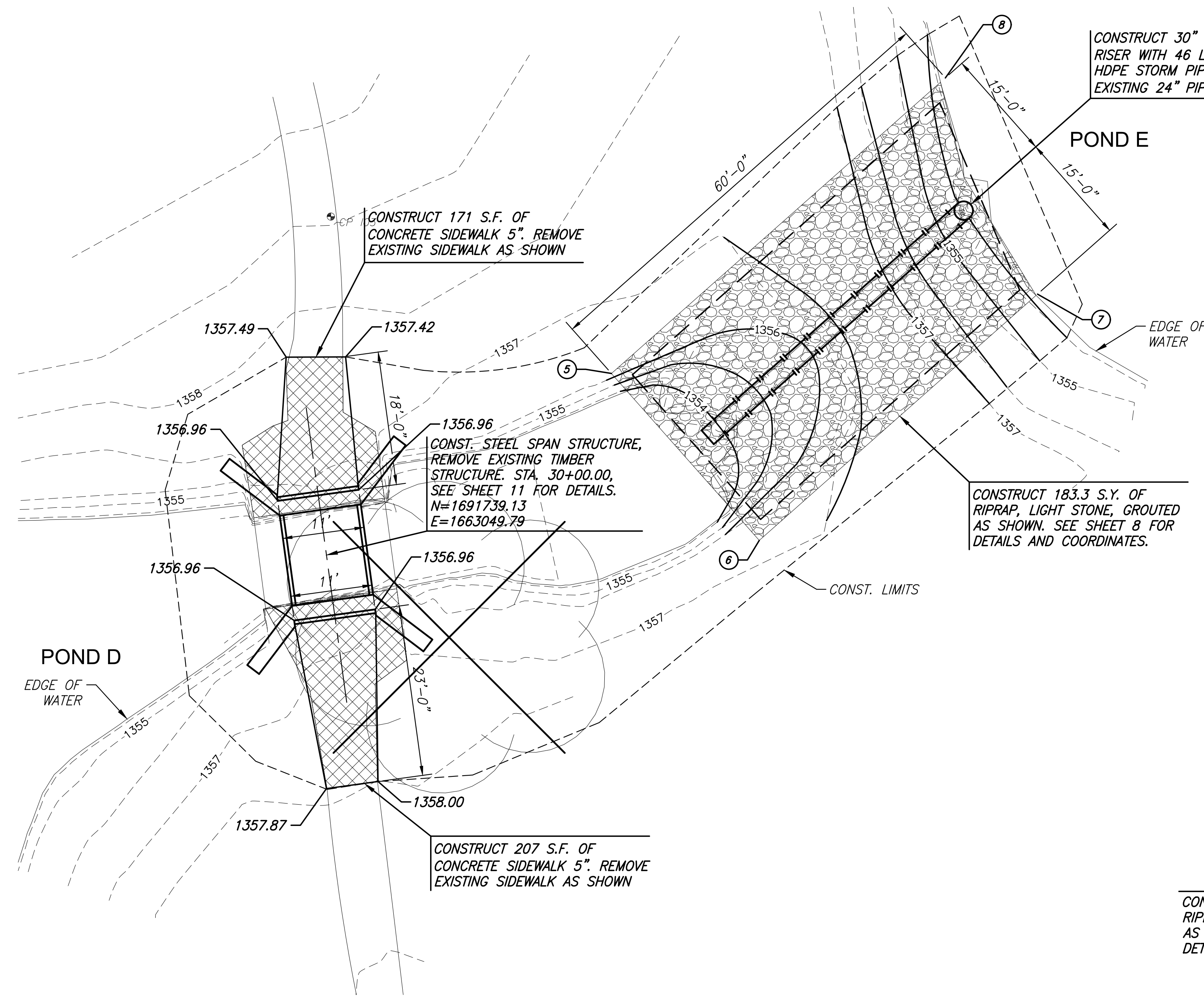
POND D & E SITE PLAN
