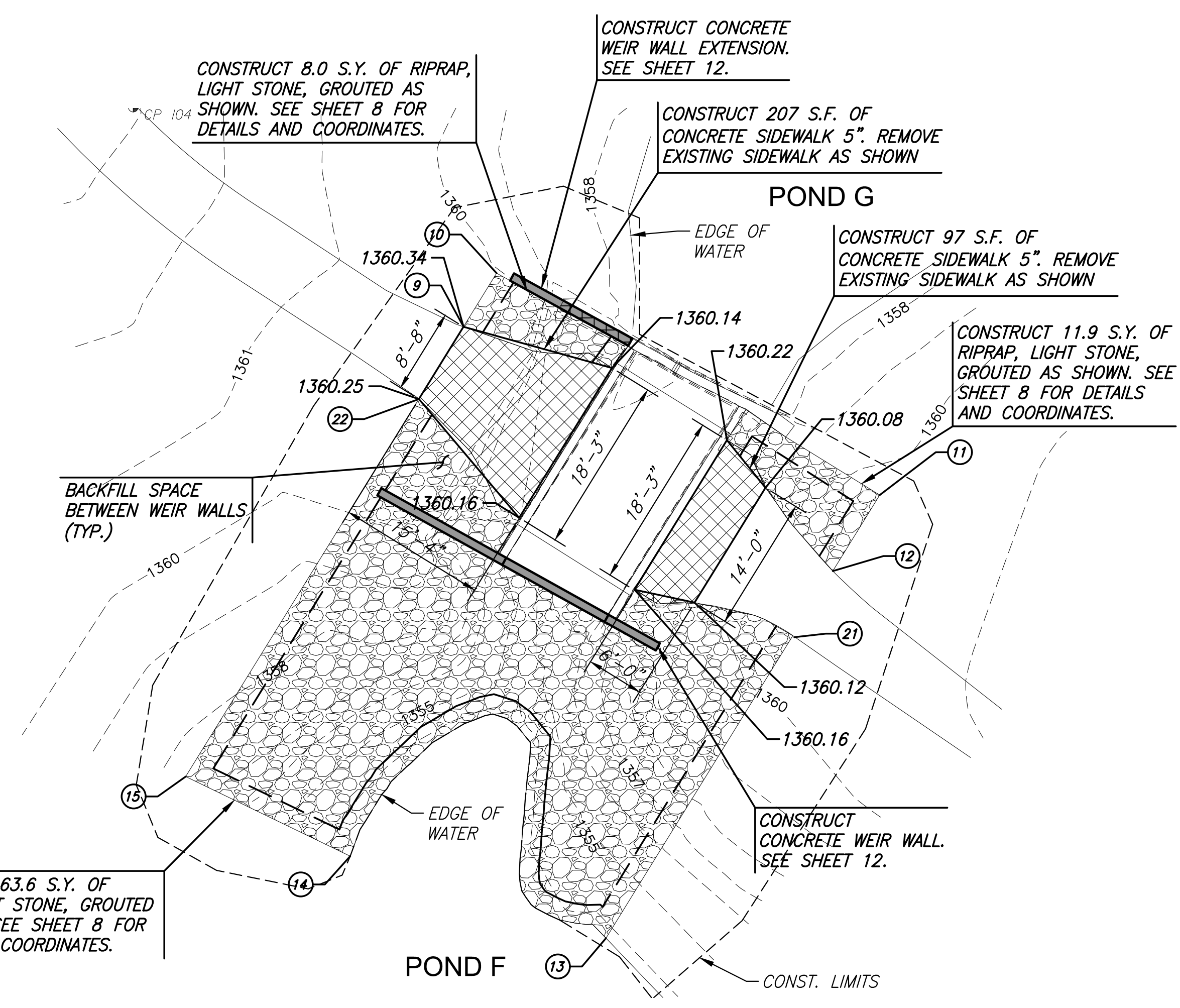
POND F & G SITE PLAN
