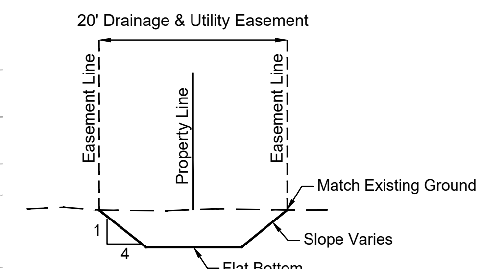
EASEMENT GRADING A-A (2) (NOT TO SCALE)
