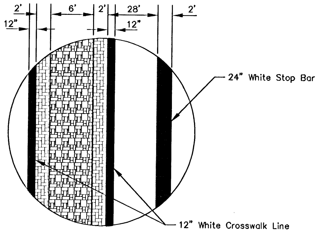
School Crossing Detail
