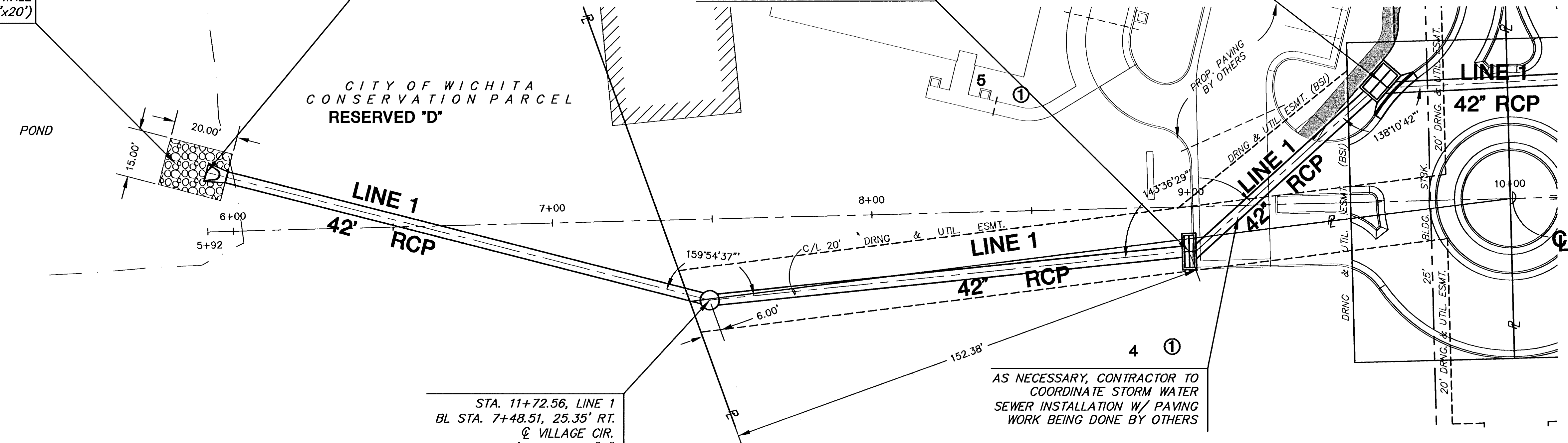
PLAN LINE 1 SCALE: 1"=20'
