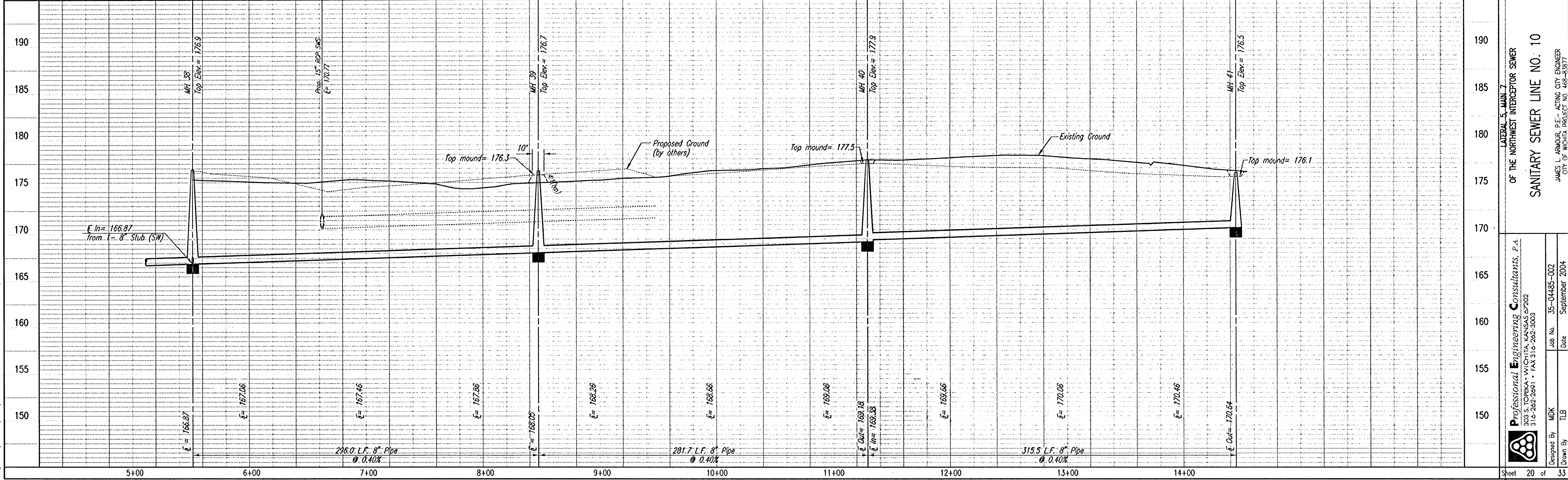
SANITARY SEWER LINE NO. 10
