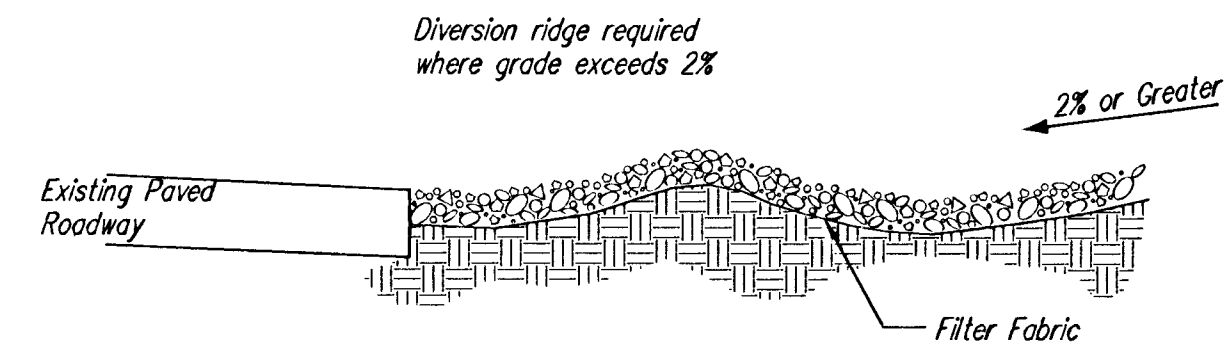
SECTION C-C
