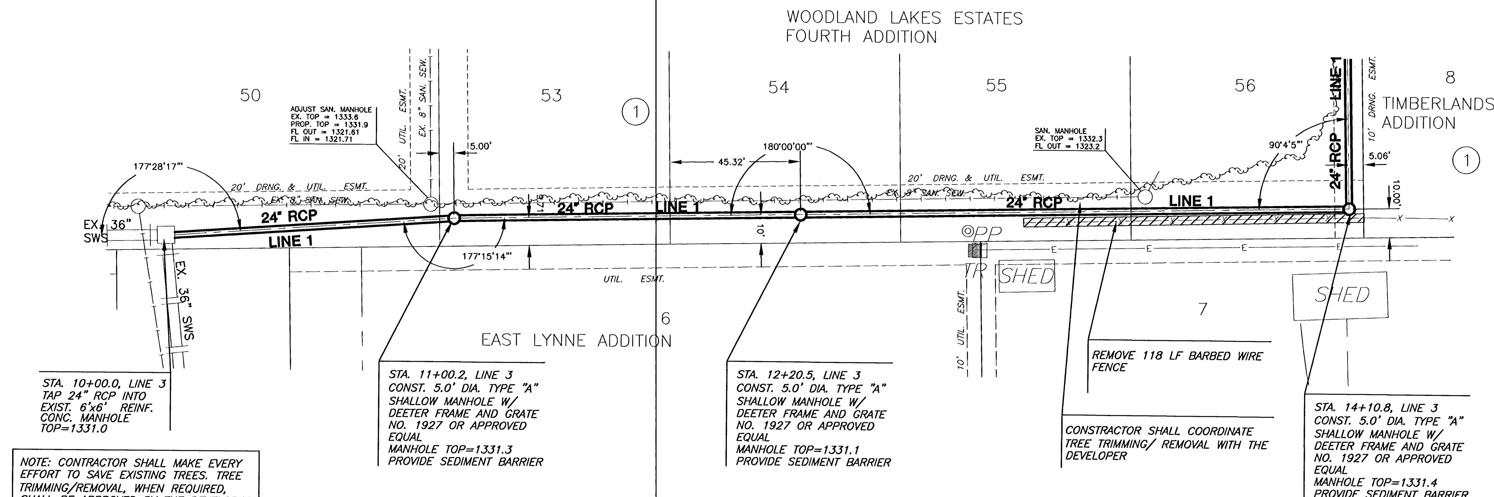
PLAN LINE 3
