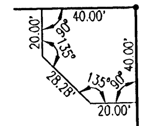
TYPICAL ENTRY MONUMENT RESERVE DETAIL
