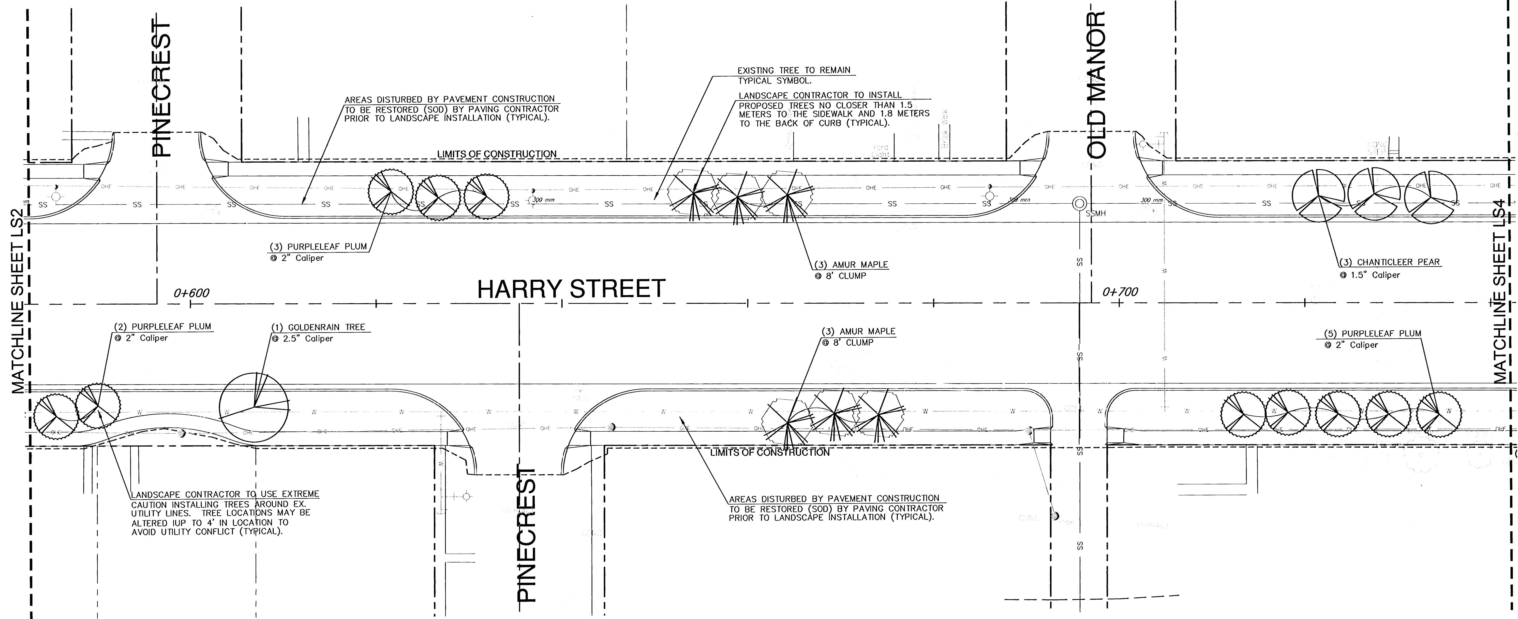
STREET PLANTING PLAN SCALE: 1:200
