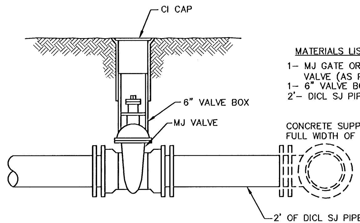
VALVE ASSEMBLY
