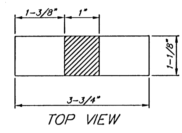
PICKHOLE DETAIL
