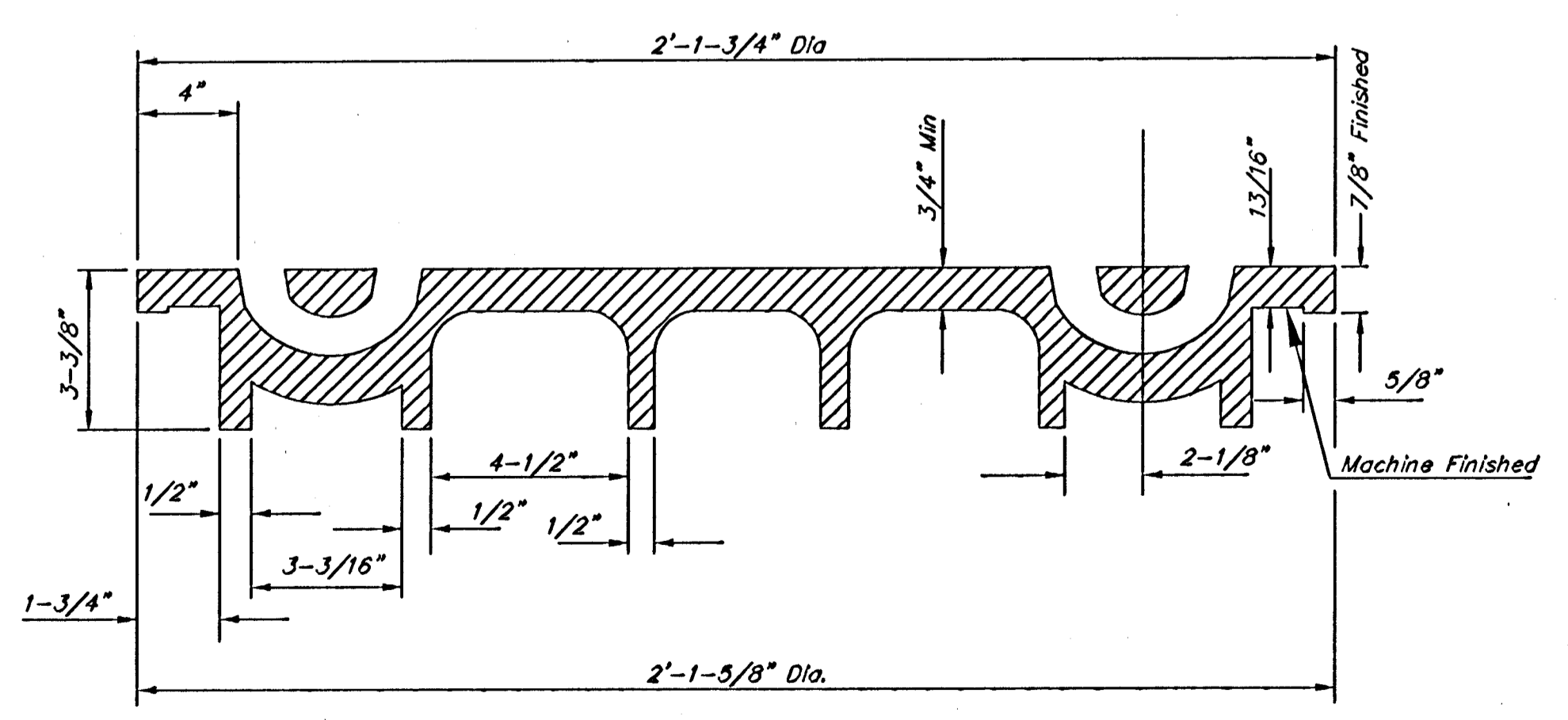
SECTION VIEW
