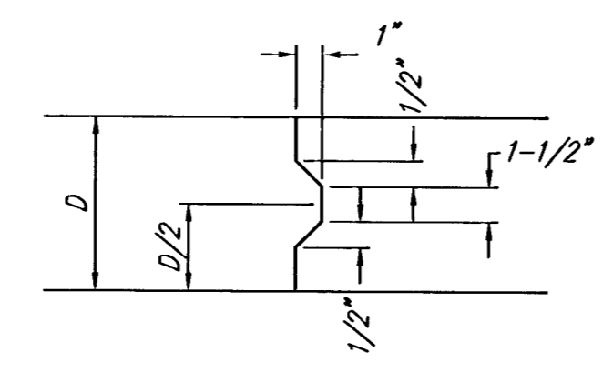
KEYWAY DETAIL
