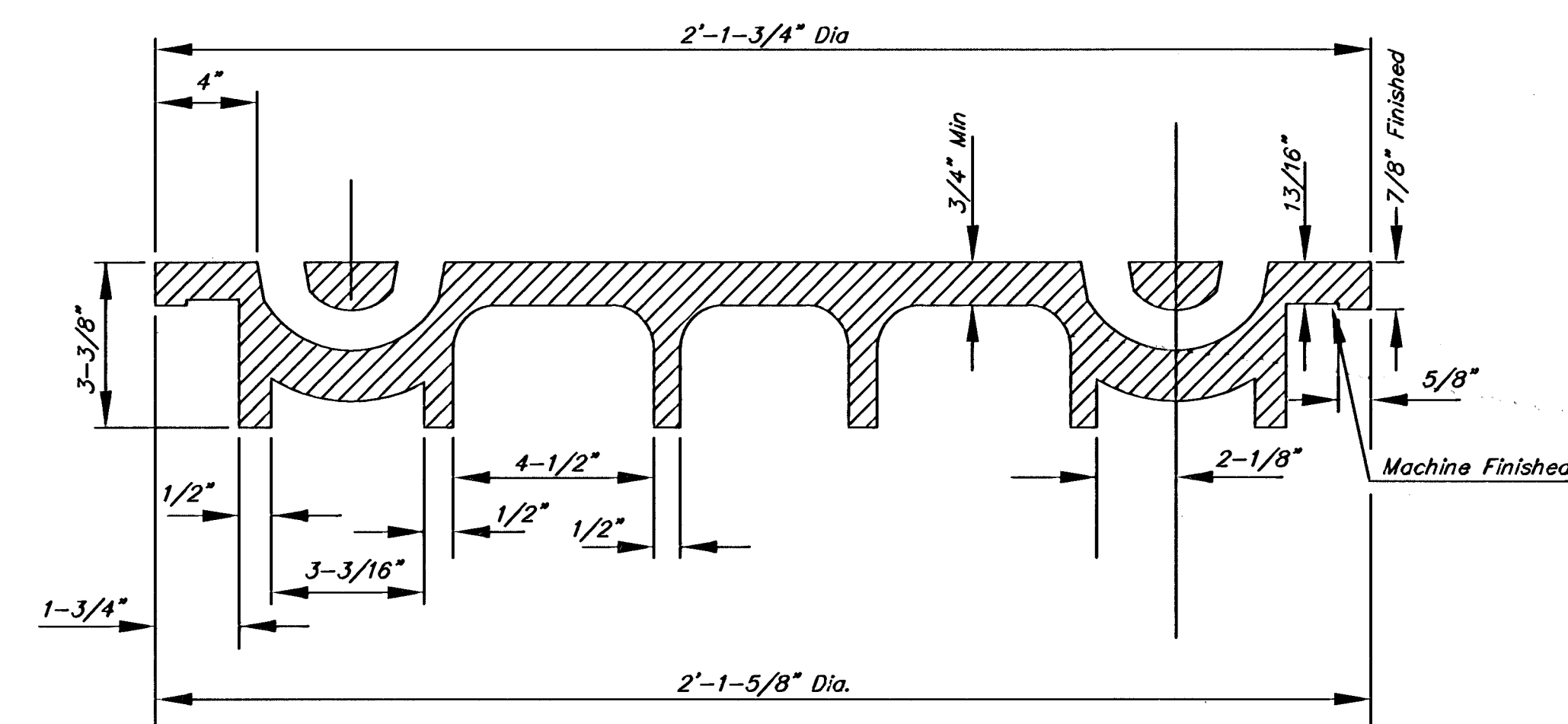
SECTION VIEW
