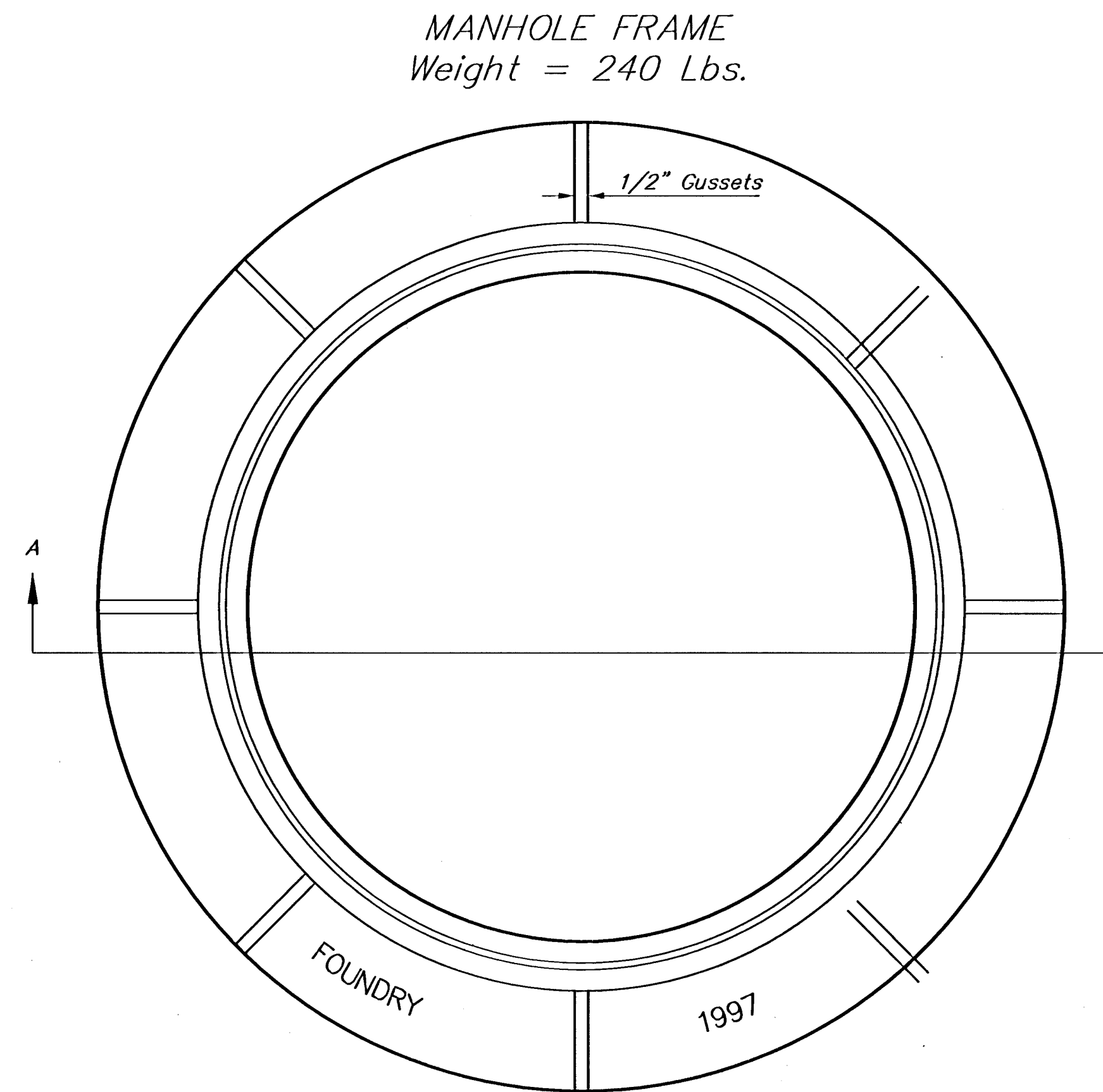
TOP VIEW
