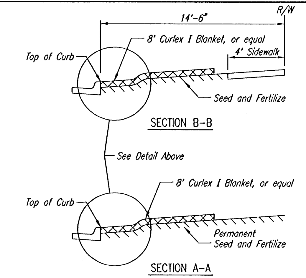
CURB BACKFILL DETAIL
