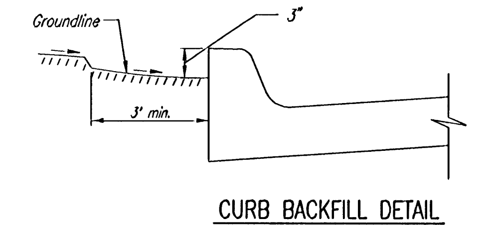
CURB BACKFILL DETAIL
