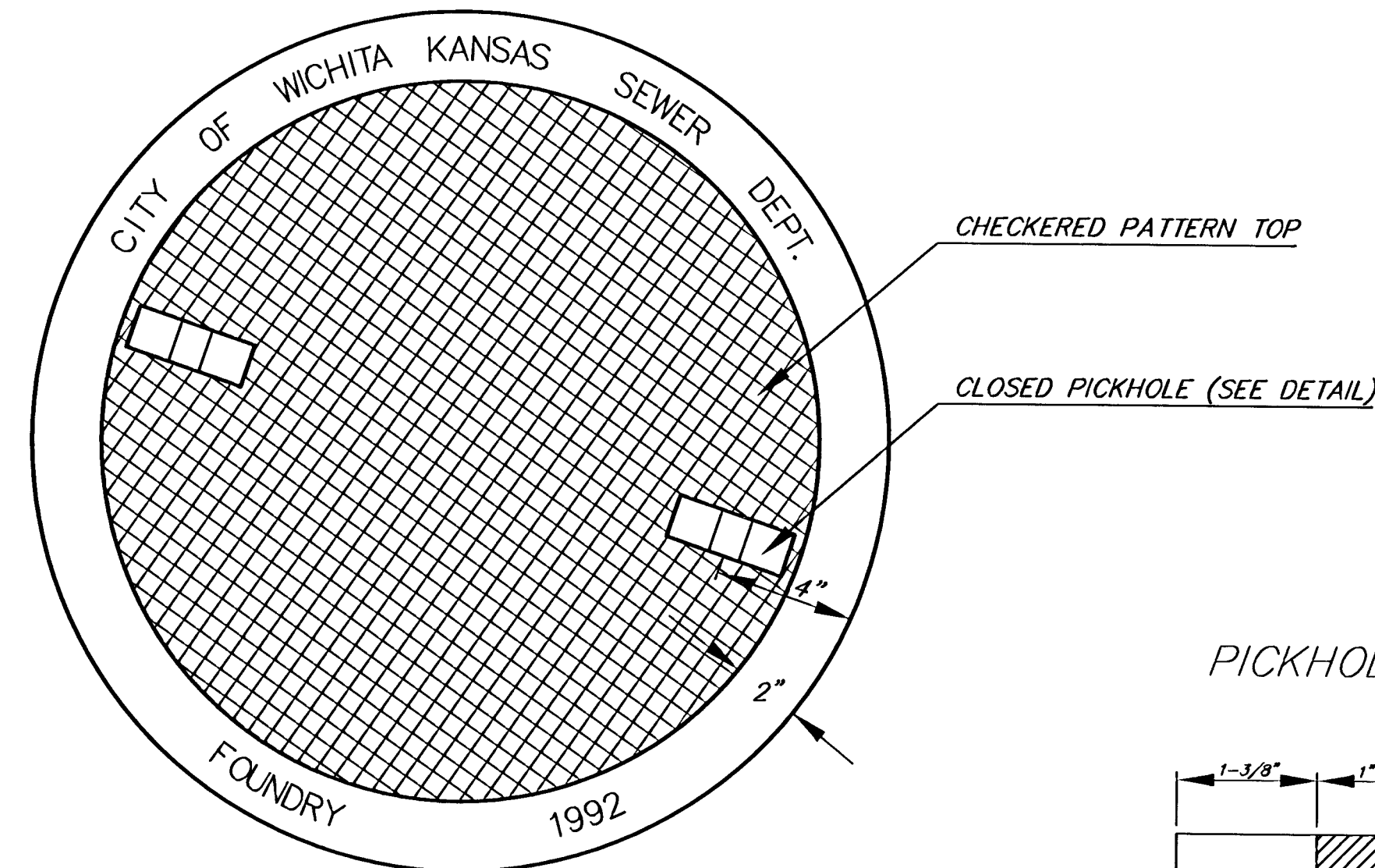
TOP VIEW
