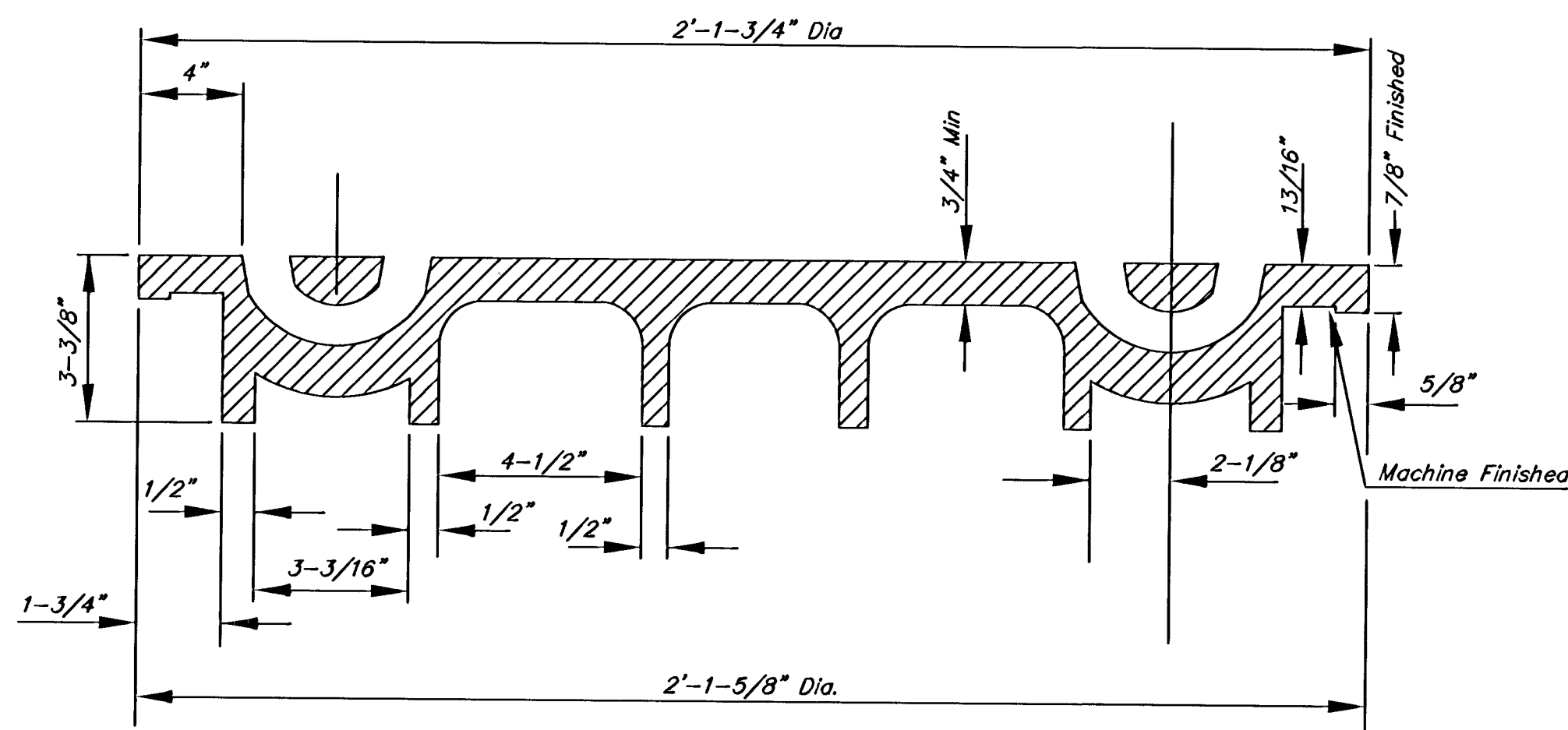
SECTION VIEW
