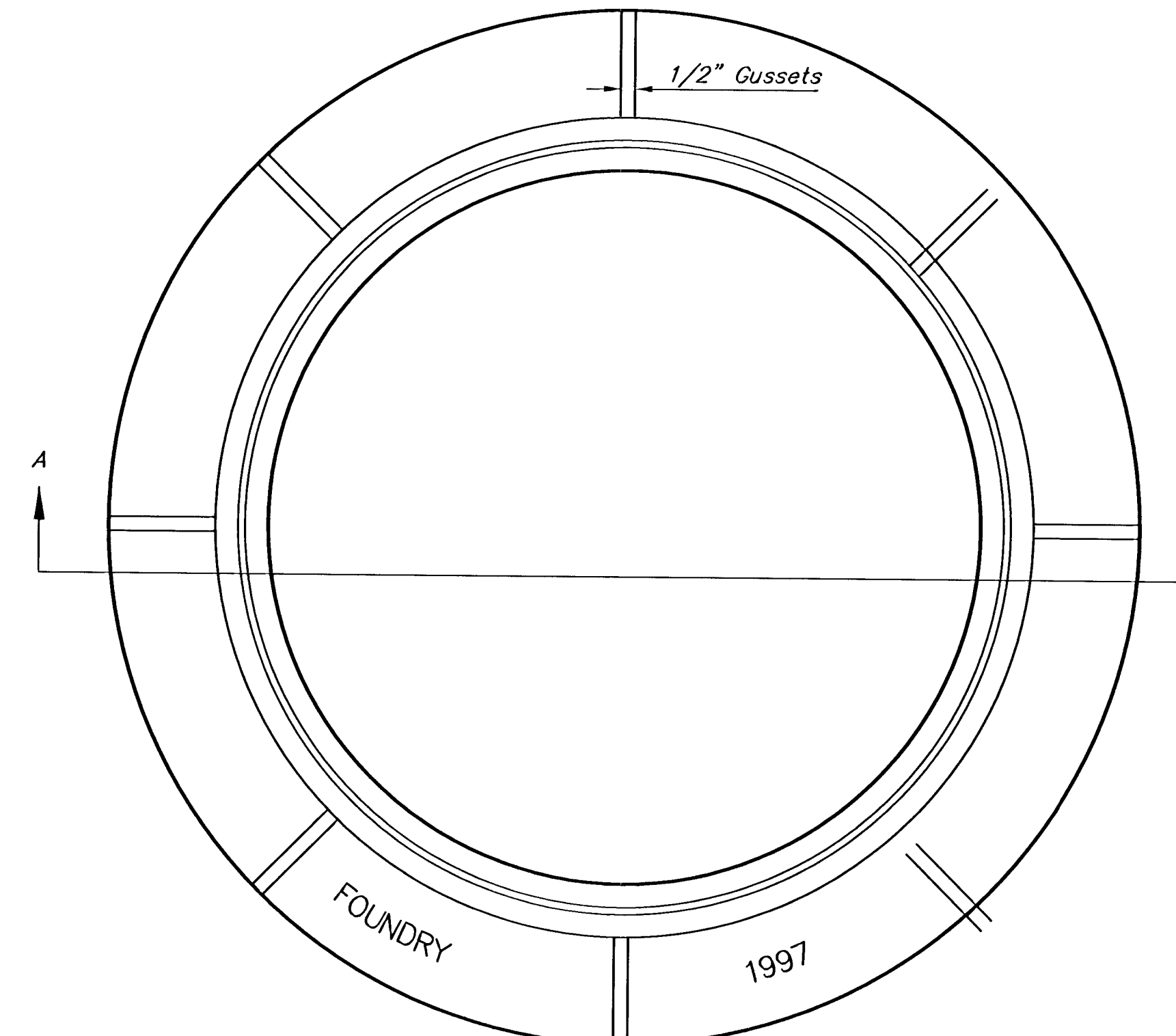
TOP VIEW
