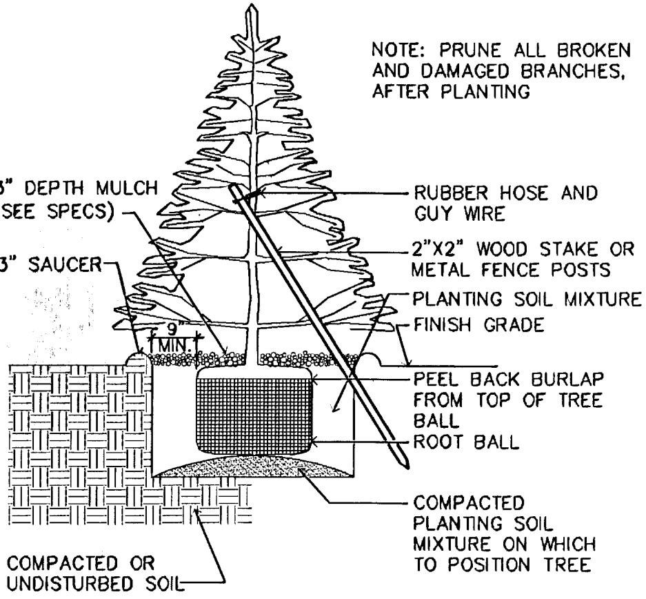
2 EVERGREEN TREE PLANTING DETAIL NOT TO SCALE
