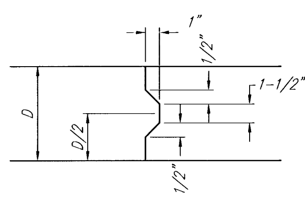
KEYWAY DETAIL
