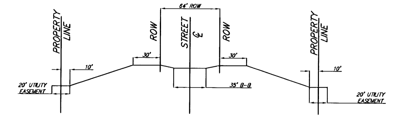
TYPICAL LOT SECTION
