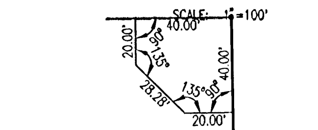
TYPICAL ENTRY MONUMENT RESERVE DETAIL
