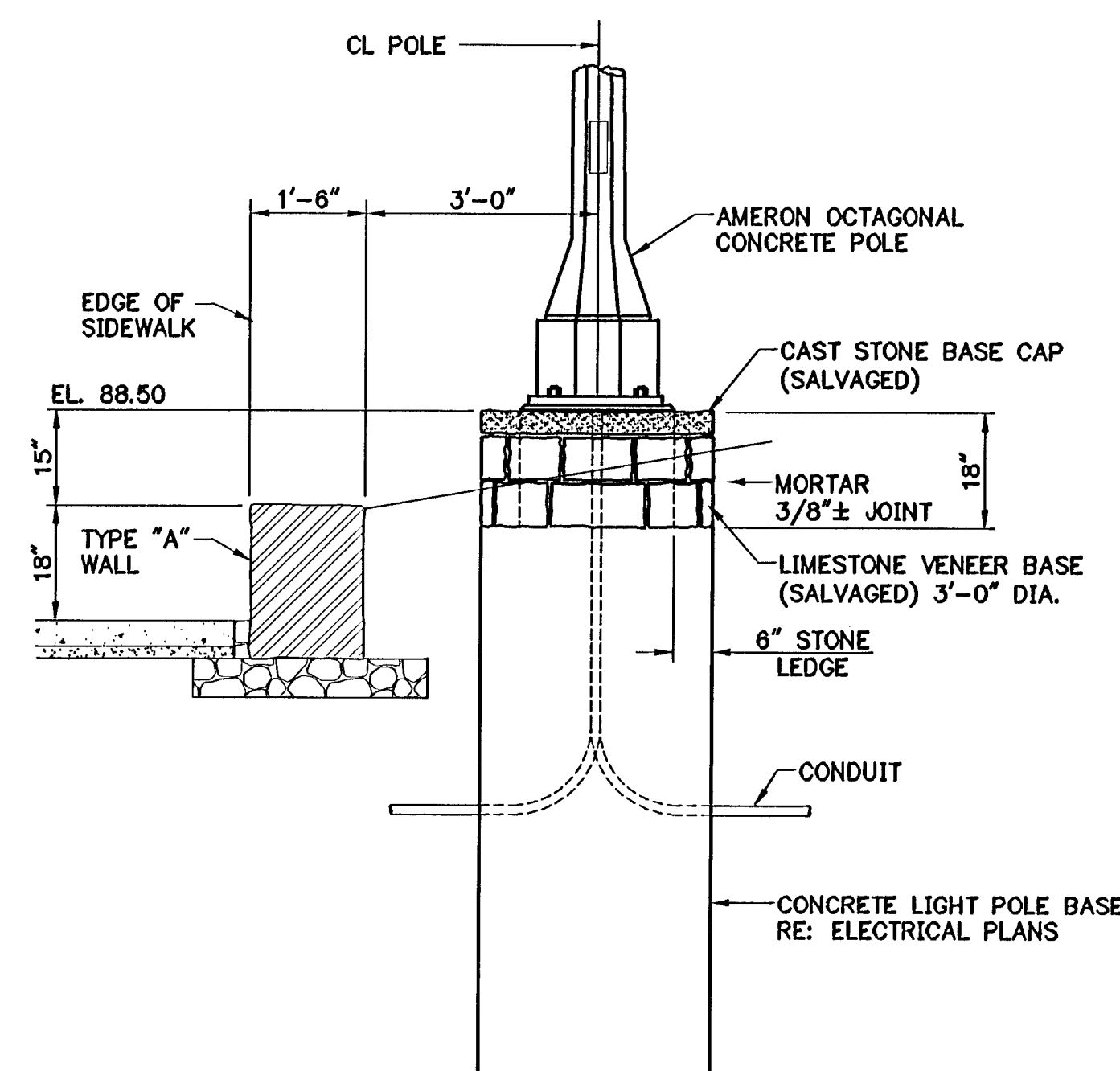
TYPE "C" LIGHT POLE BASE DETAIL (LOCATED BEHIND WALL) SCALE: 1/2"-1'-0"
