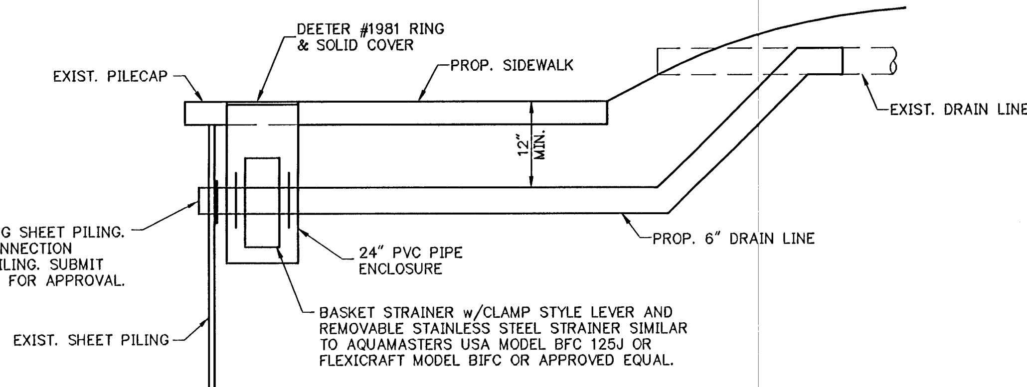
STRAINER DETAIL
