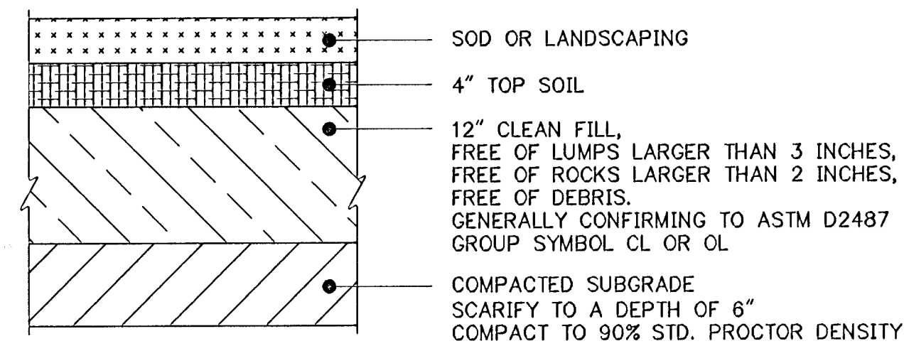
FINISH GRADE SECTION
