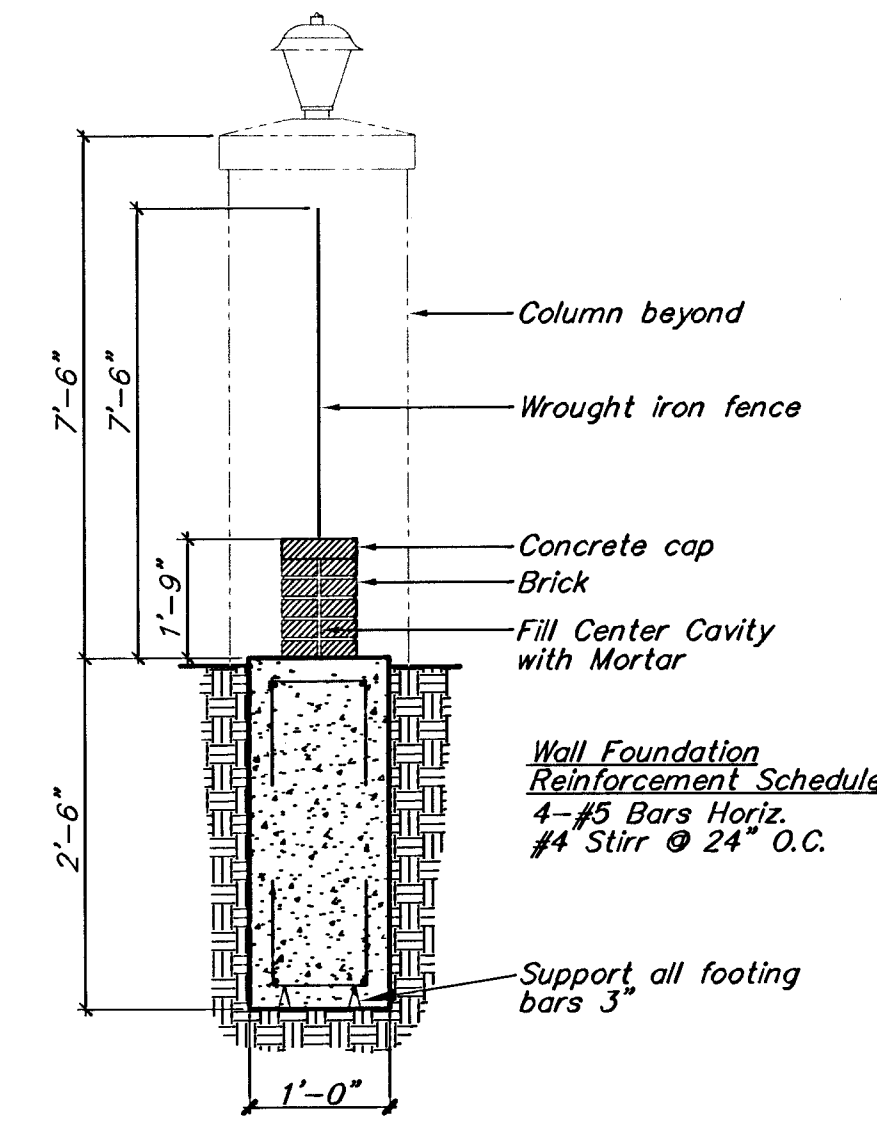
MAJOR WALL SECTION NO SCALE
