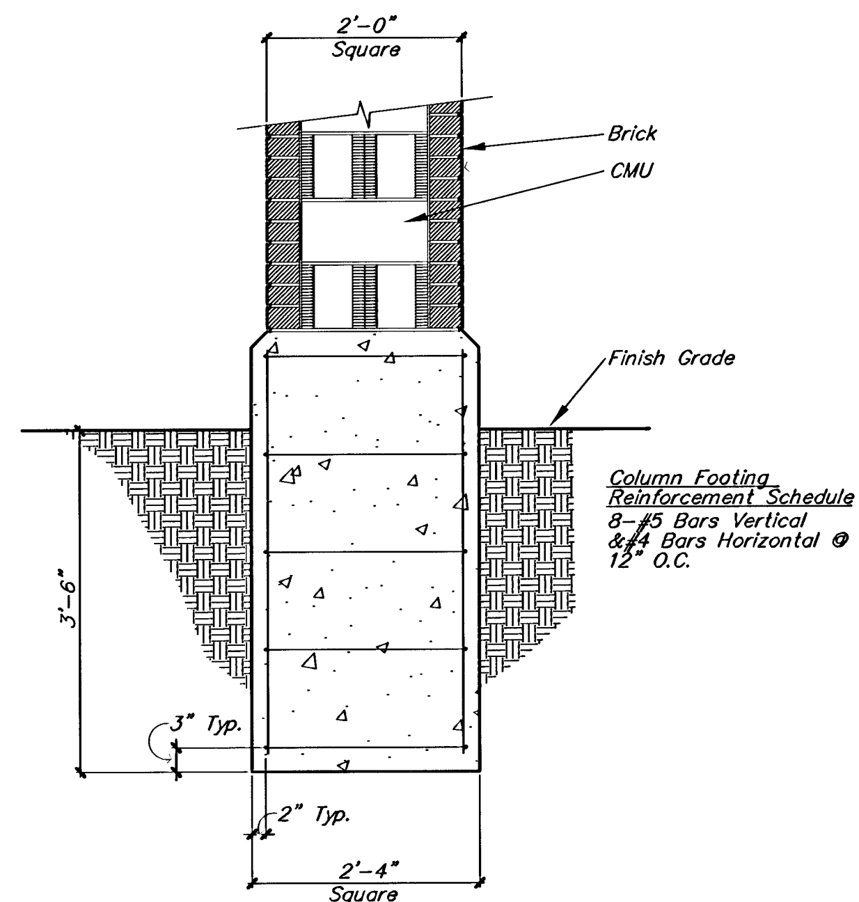
COLUMN SECTION & FOOTING NO SCALE
