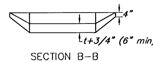
STANDARD WHEELCHAIR RAMP DETAIL NO SCALE
