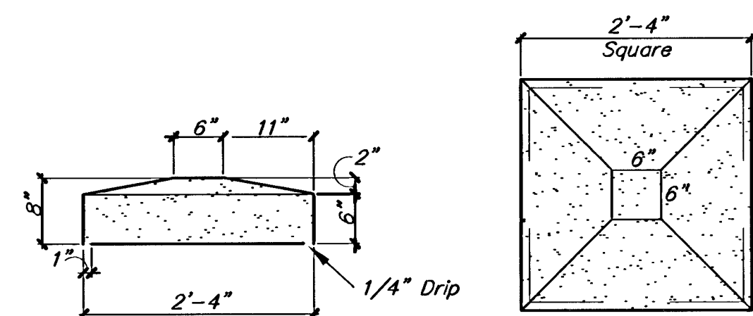
PLAN & SECTION CONCRETE CAP & PIER NO SCALE
