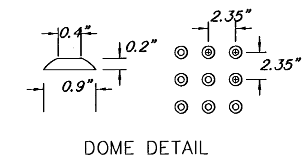
DOMES DETAIL
