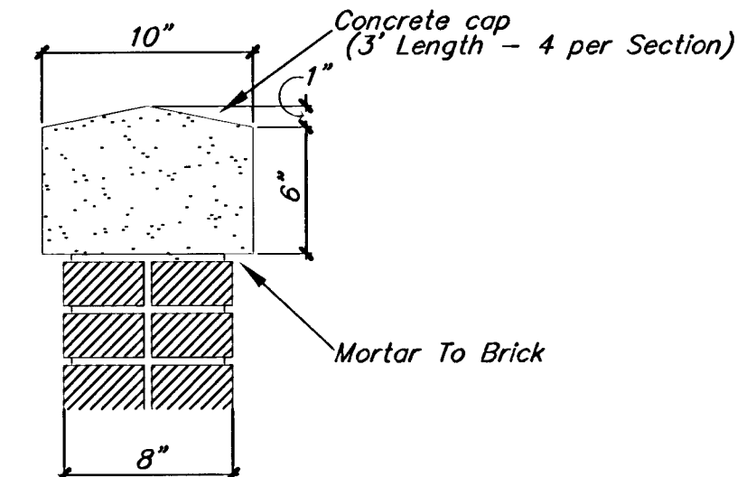
CONCRETE CAP NO SCALE
