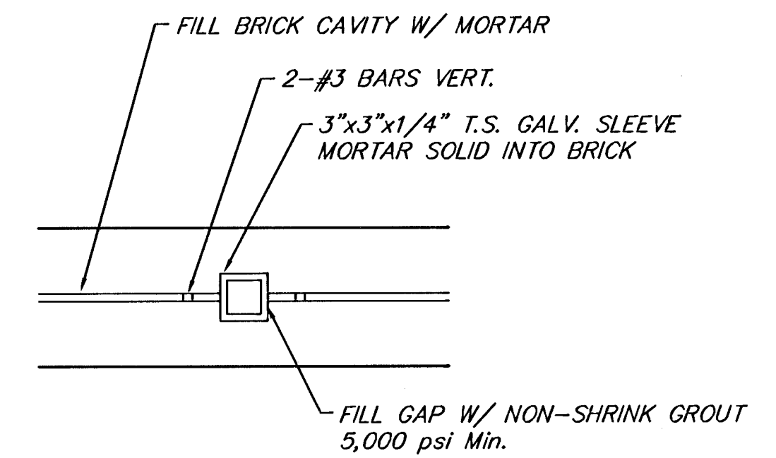
SLEEVE PLAN FOR CENTER POST NO SCALE
