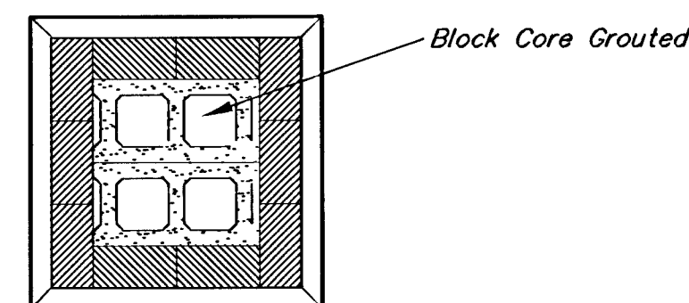
COLUMN BLOCK PLAN NO SCALE
