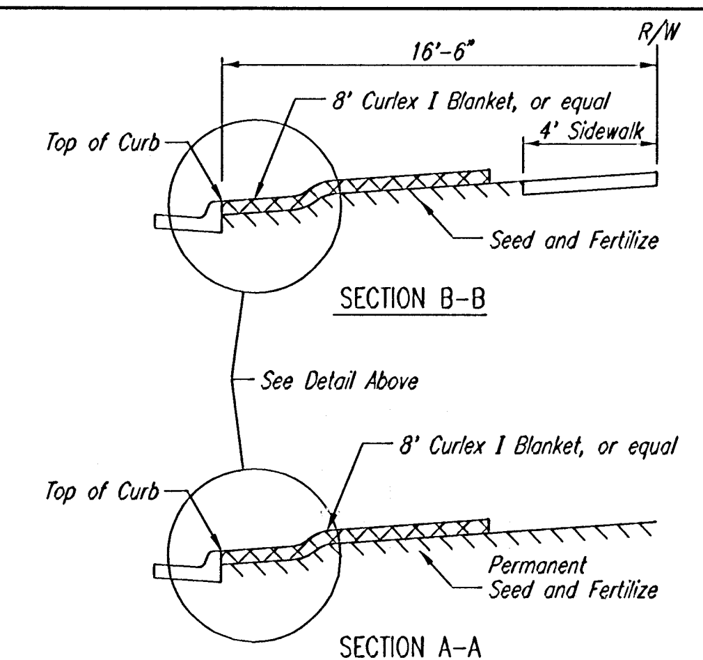
CURB BACKFILL DETAIL
