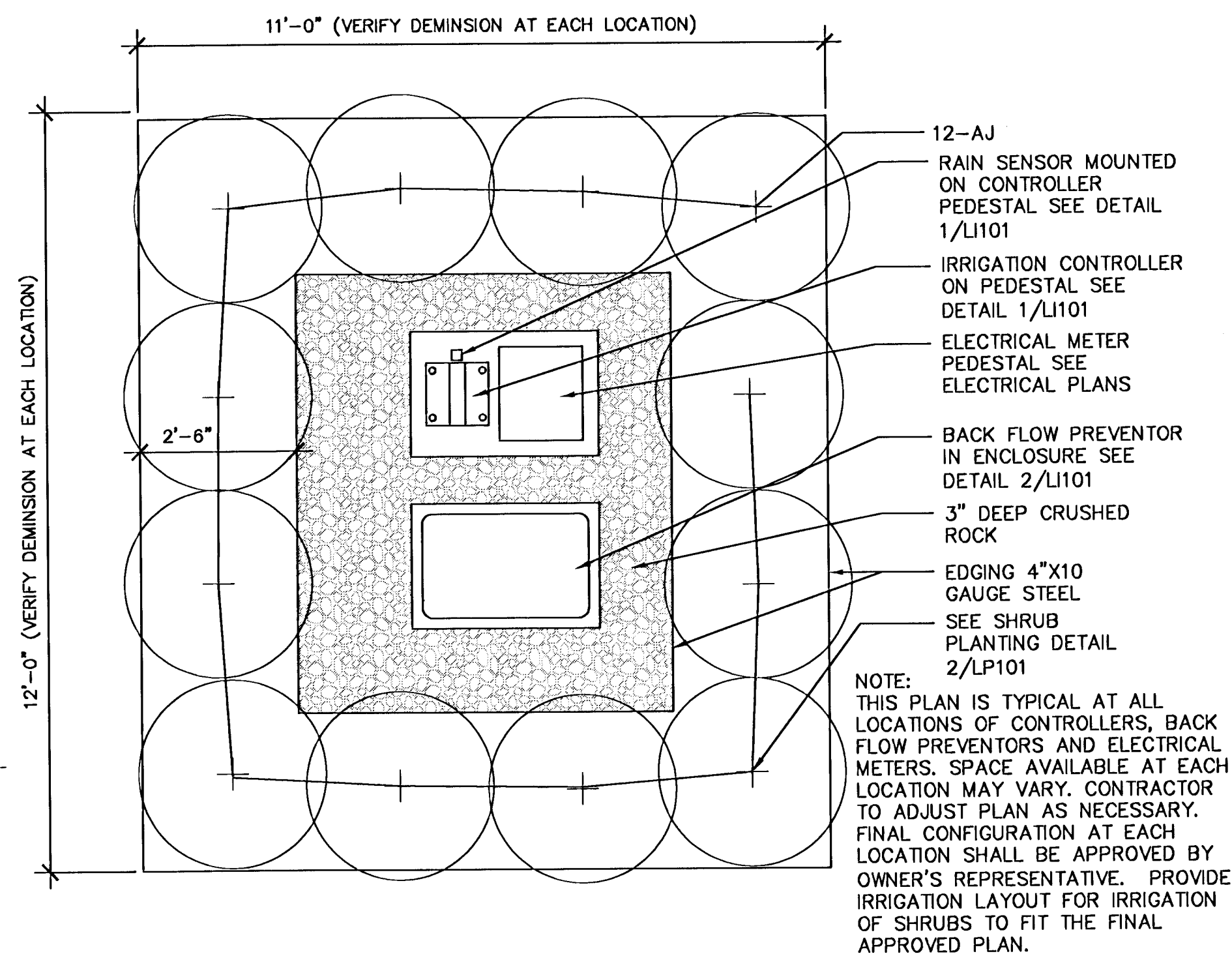
2 TYP. PLANTING AT CONTROLLER & BACKFLOW PREVENTOR
