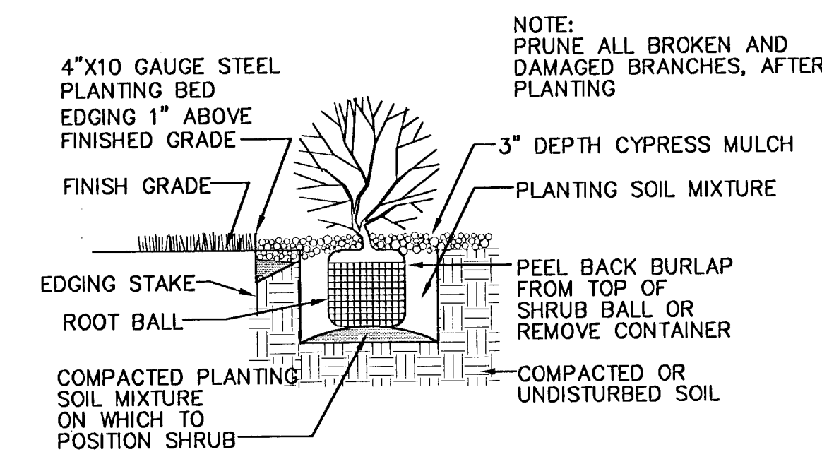
3 SHRUB PLANTING DETAIL
