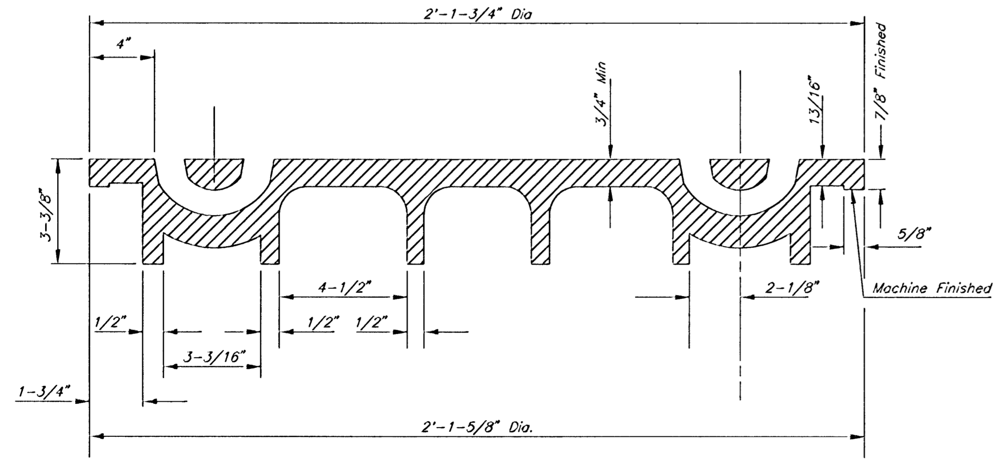
SECTION VIEW
