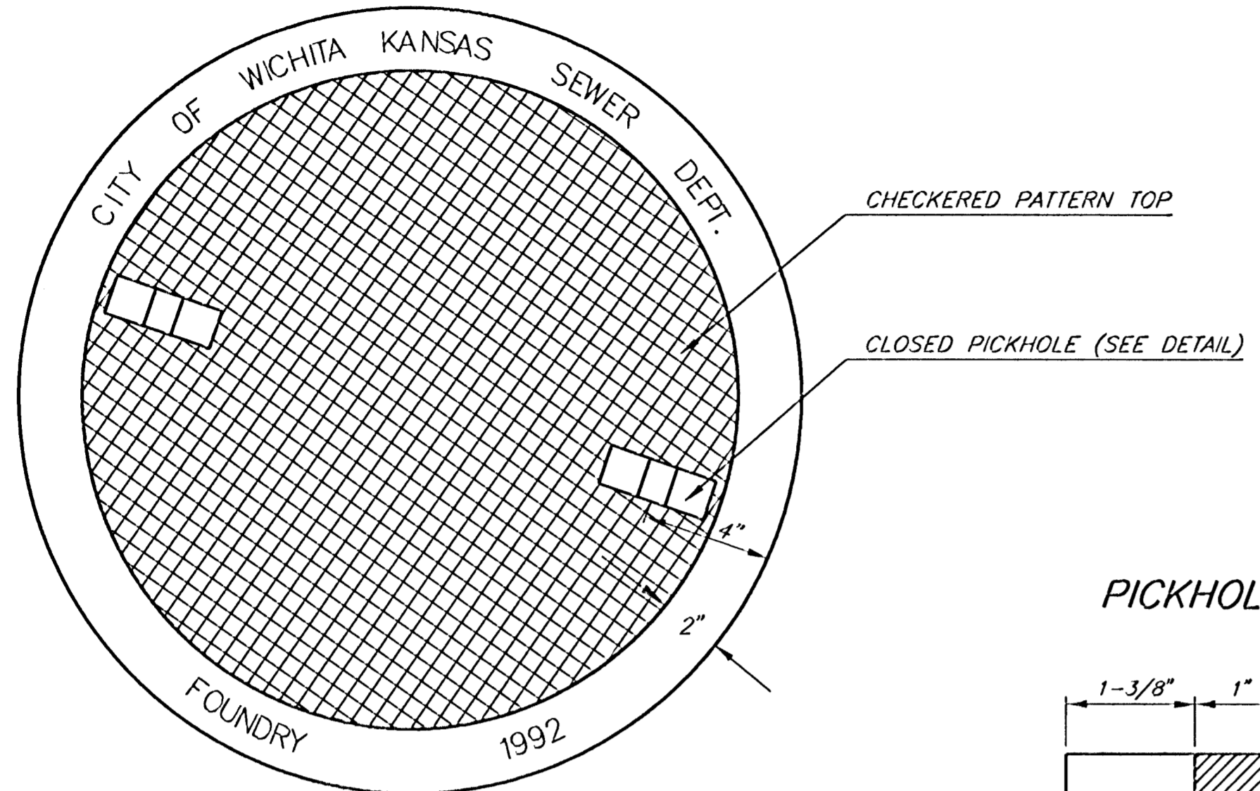
TOP VIEW
