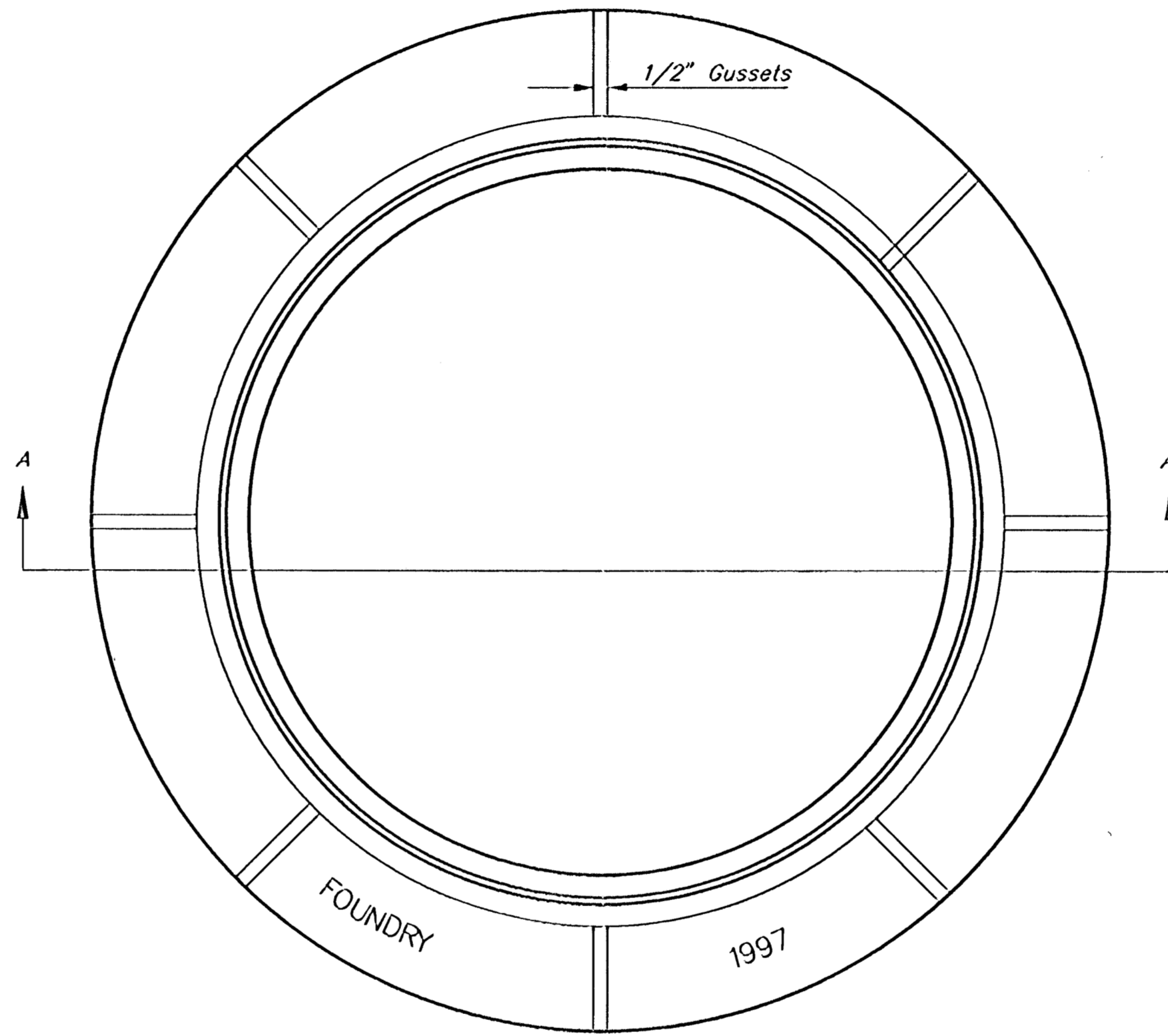
TOP VIEW
