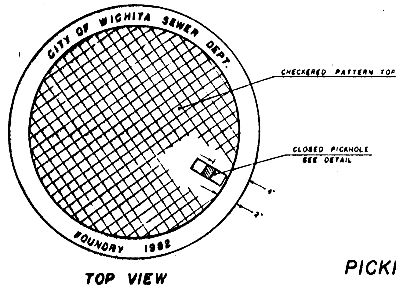
TOP VIEW
