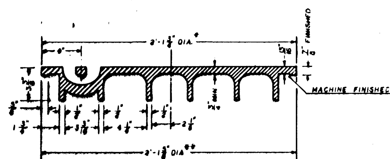
SECTION VIEW
