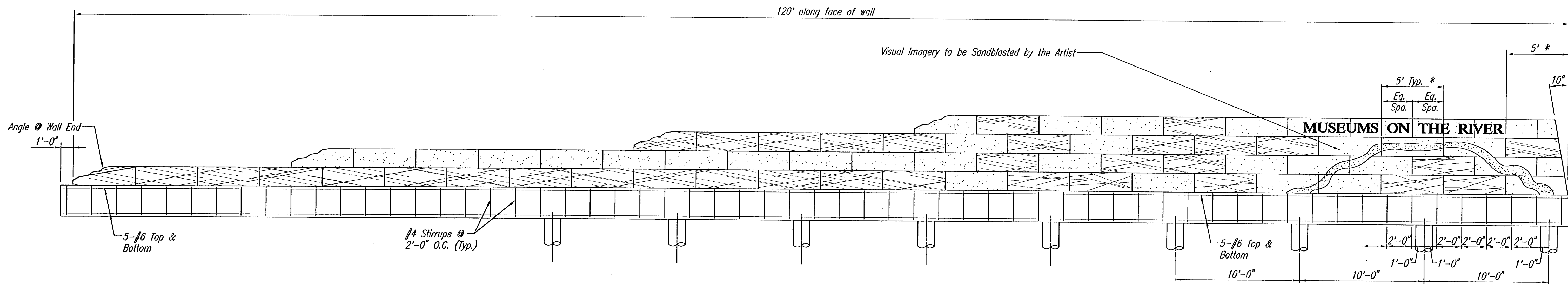
(B) WALL ELEVATION
