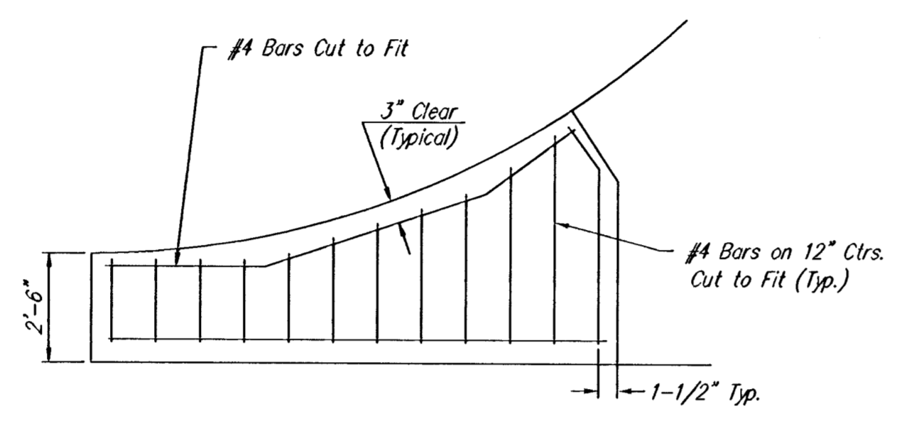
WING REINFORCING DETAIL
