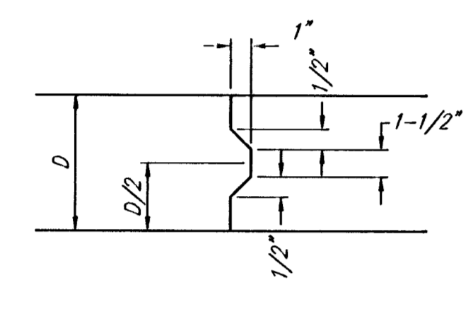
KEYWAY DETAIL
