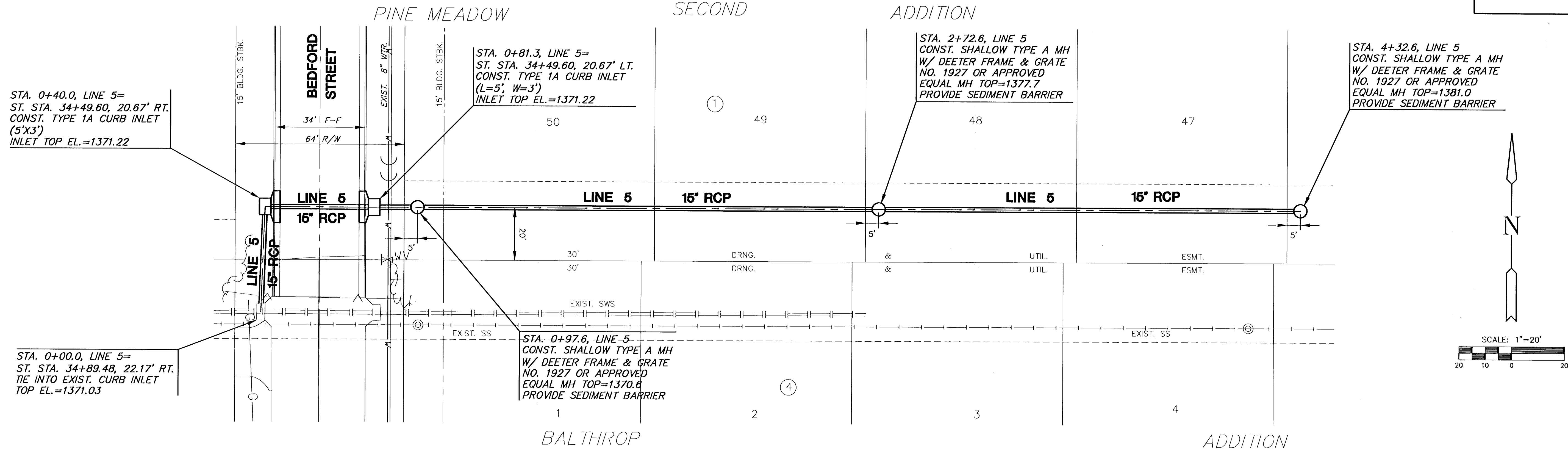
PLAN LINE 5 SCALE: 1"=20'
