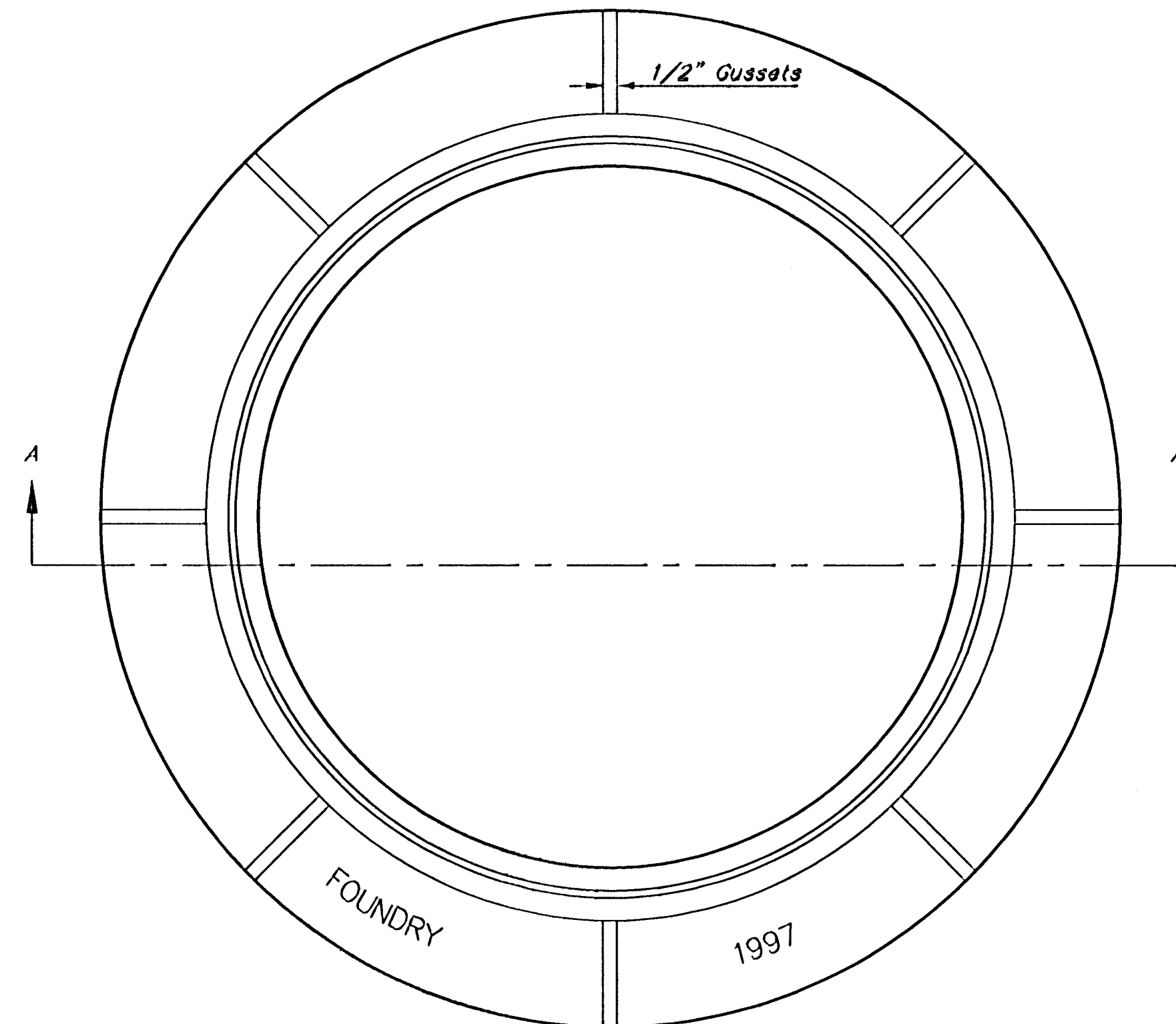
TOP VIEW
