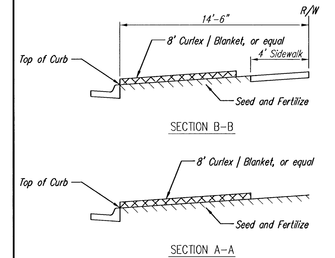
CURB BACKFILL DETAIL
