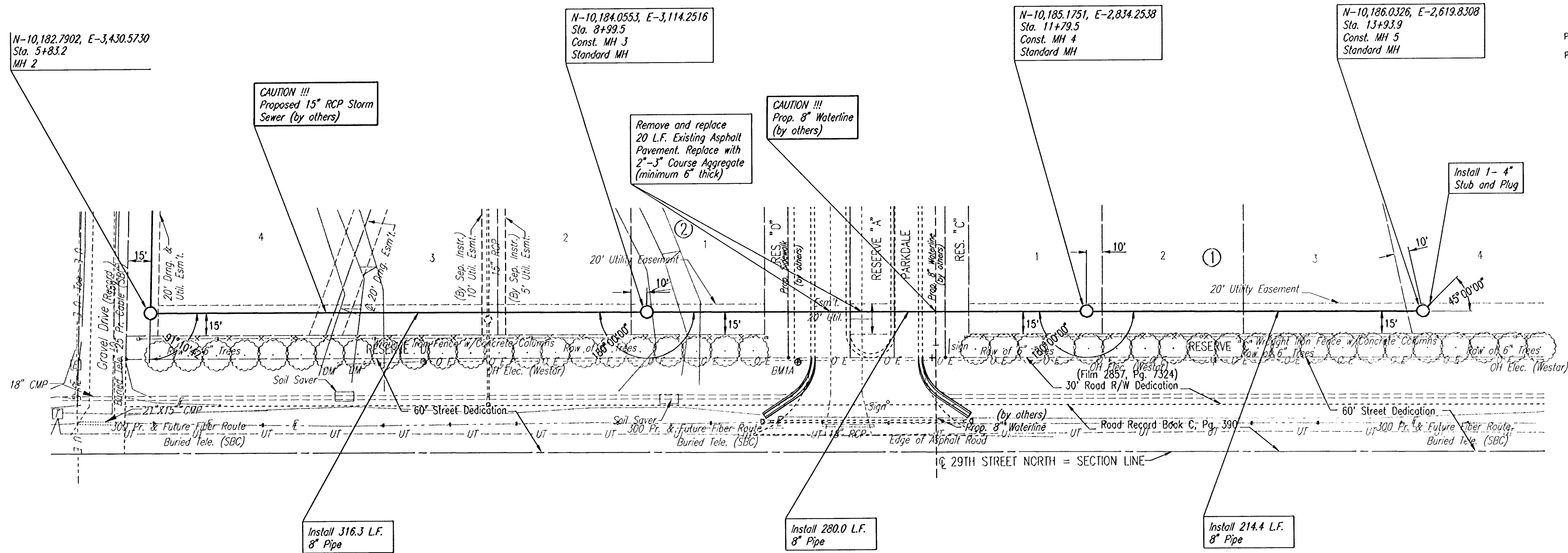
SANITARY SEWER LINE NO. 1
