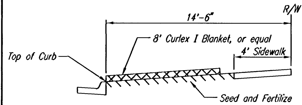
SECTION B-B
