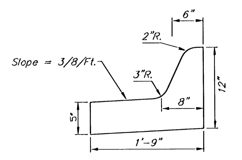
Medial Curb Detail (Low Edge) Not to Scale Note: To be paid as Medial Curb & Cutter (6 5/8")
