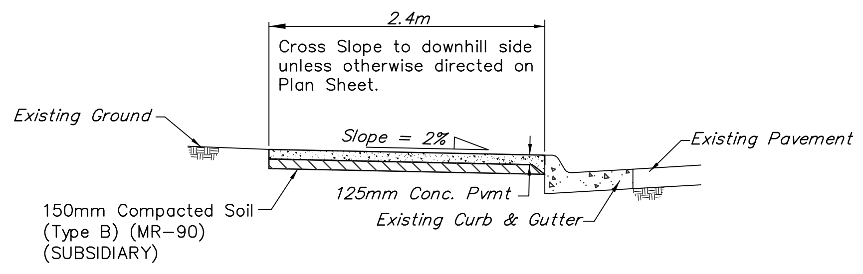
TYPICAL SECTION ADJACENT TO STREET Sta. 0+028.50 to Sta. 0+134.15, Path No. 6 NO SCALE
