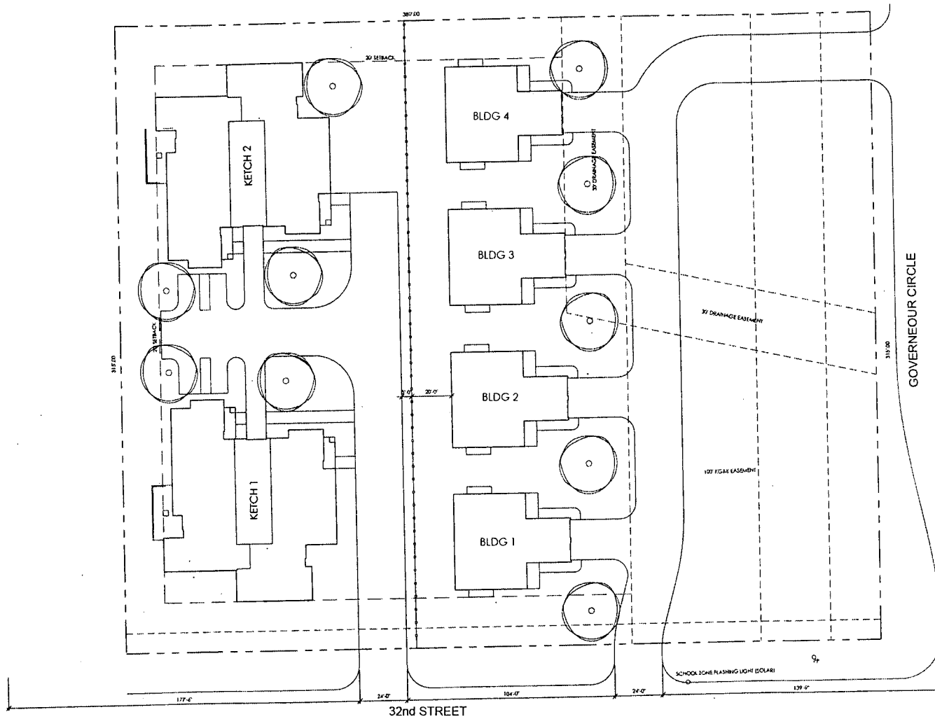
A SITE DEVELOPMENT PLAN 1"=20'-0" NORTH
