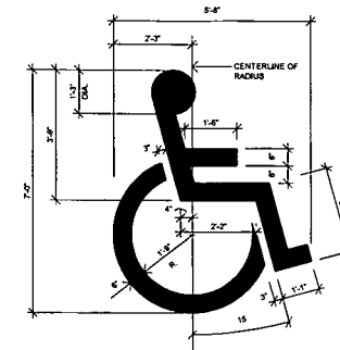
③ ACC. PARKING SYMBOL \frac{3}{8}"=1'-0" 0 2'
