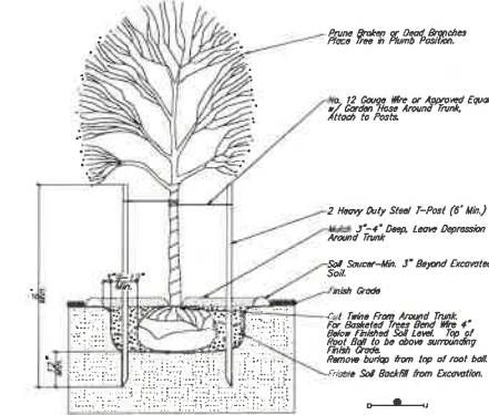
1 TREE PLANTING & STAKING DETAIL 1/8" = 1'-0" No Scale
