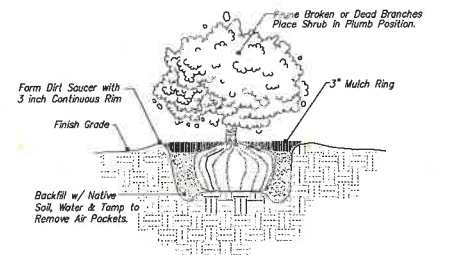
2 SHRUB PLANTING DETAIL 3/8" = 1'-0" No Scale
