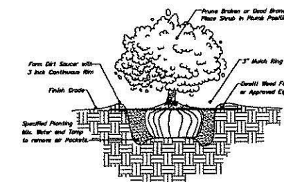
SHRUB PLANTING DETAIL 3 Gal. and Smaller No Scale
