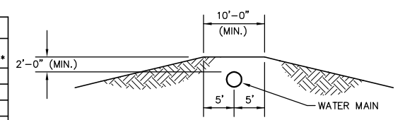
PROTECTIVE FILL DETAIL
