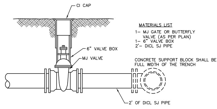
VALVE ASSEMBLY
