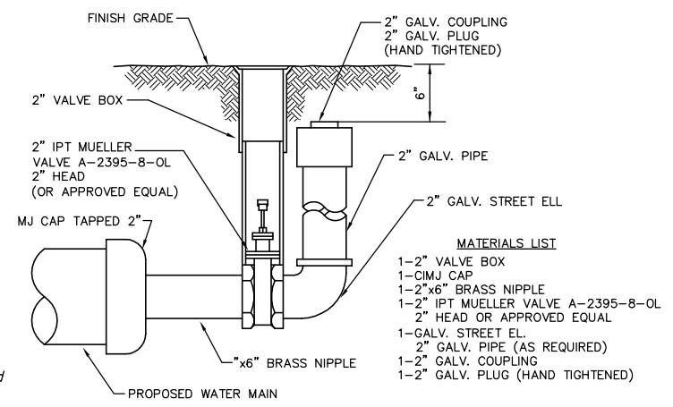
BLOWOFF ASSEMBLY 2" PER C.O.W.
