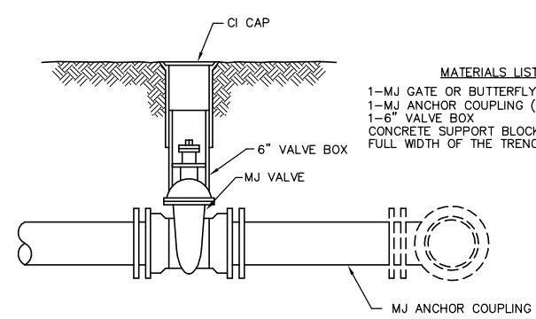
ANCHORED VALVE ASSEMBLY
