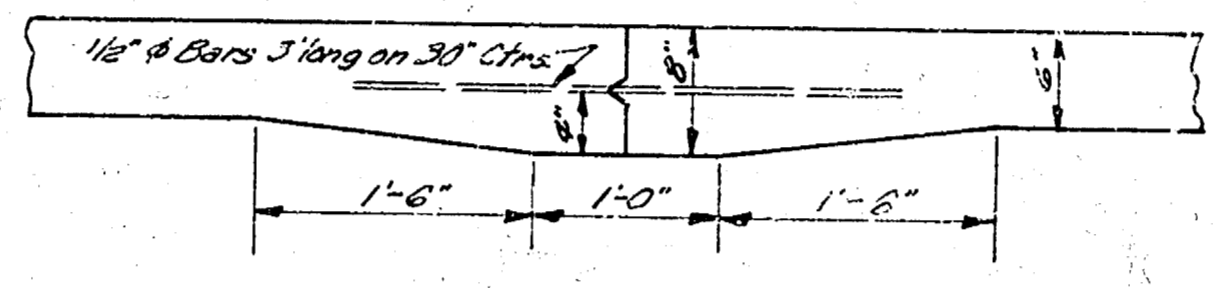
Mastic Joint Detail No Scale
