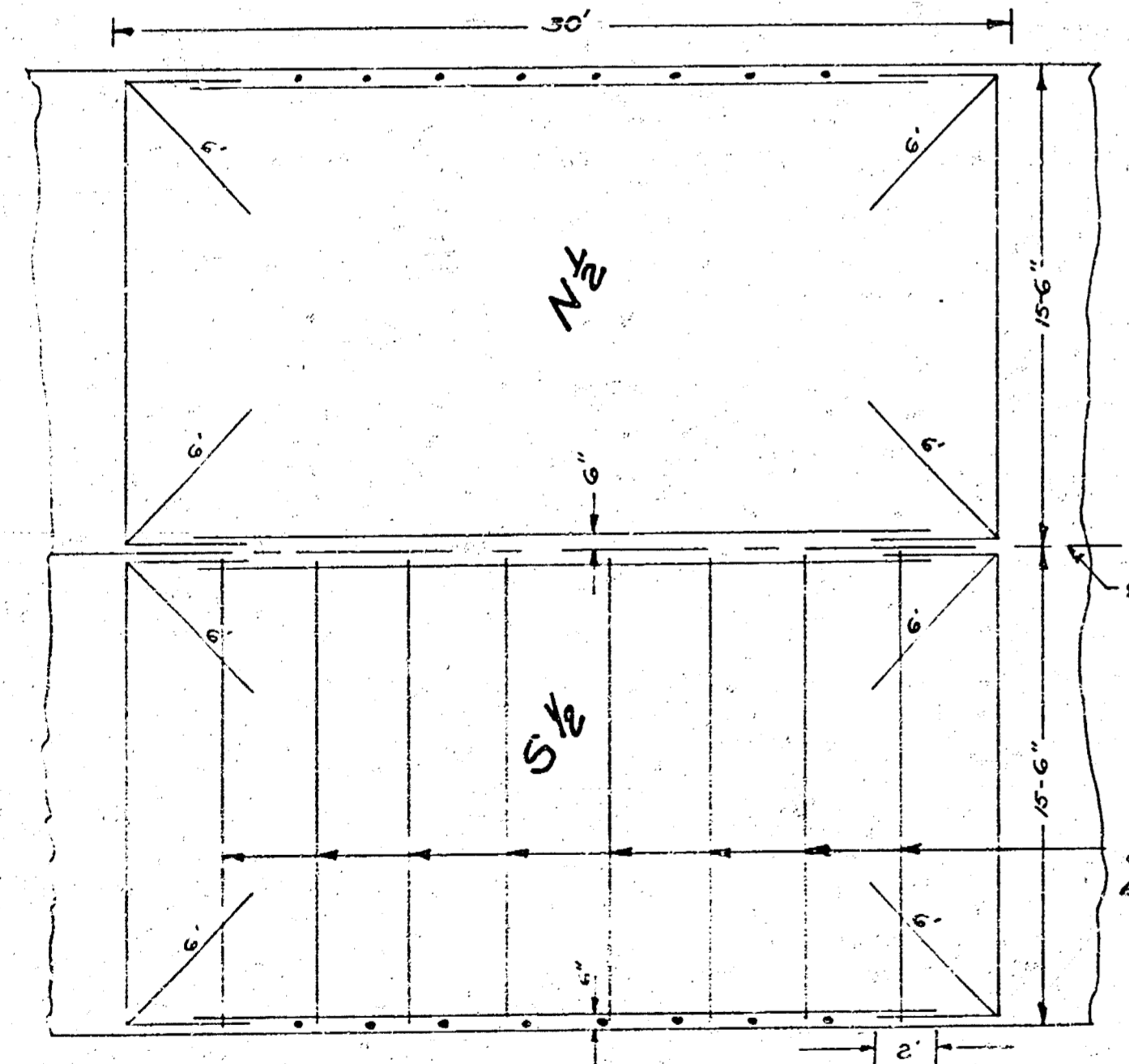
STEEL PATTERN
