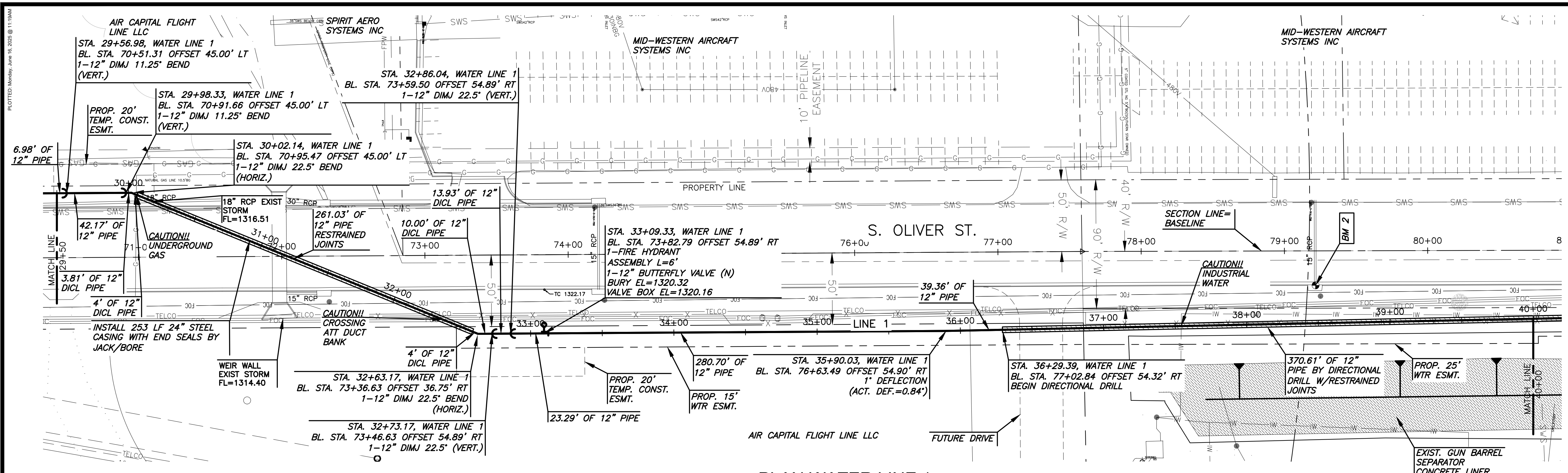
PLAN WATER LINE 1 PROFILE WATER LINE 1
