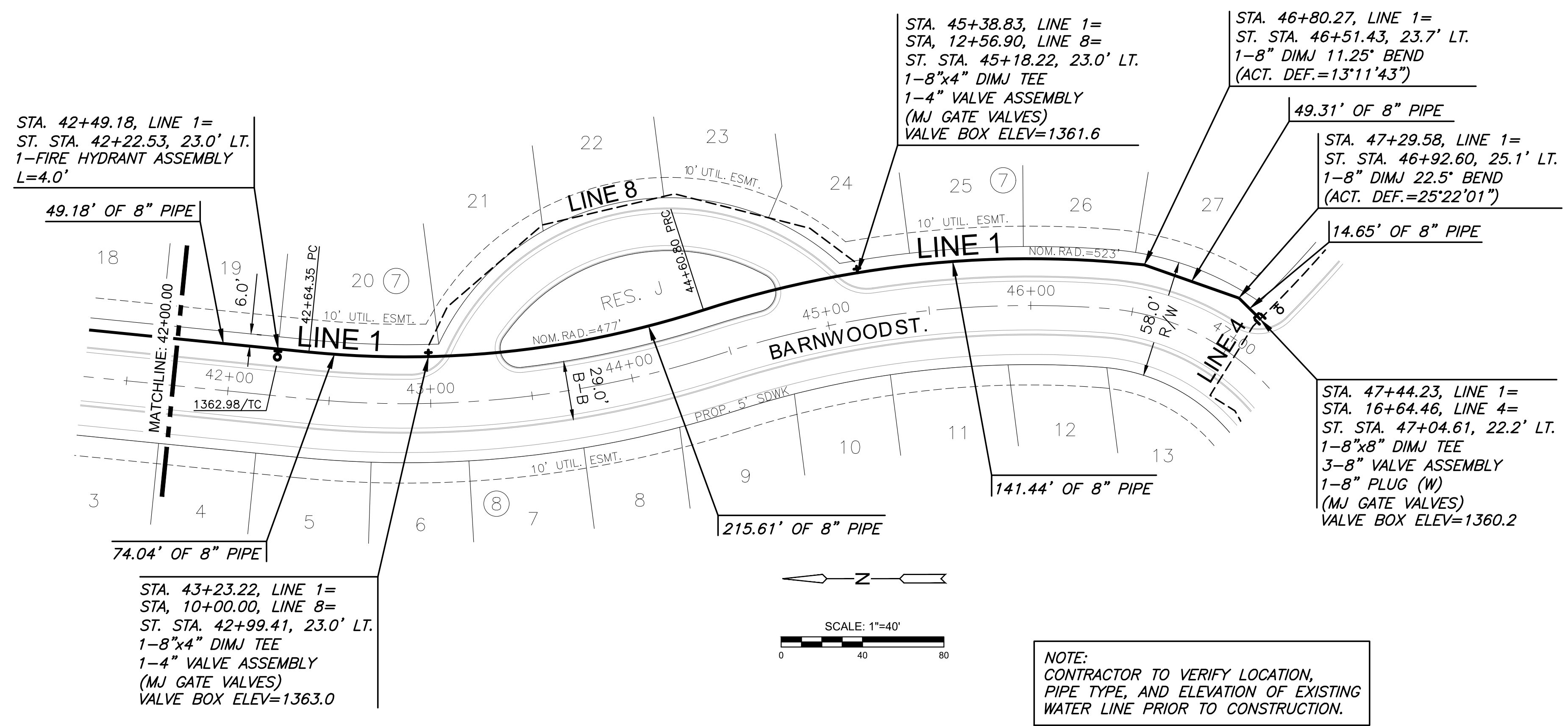
PLAN WATER LINE 1 (42+00.00 - 47+44.23)
