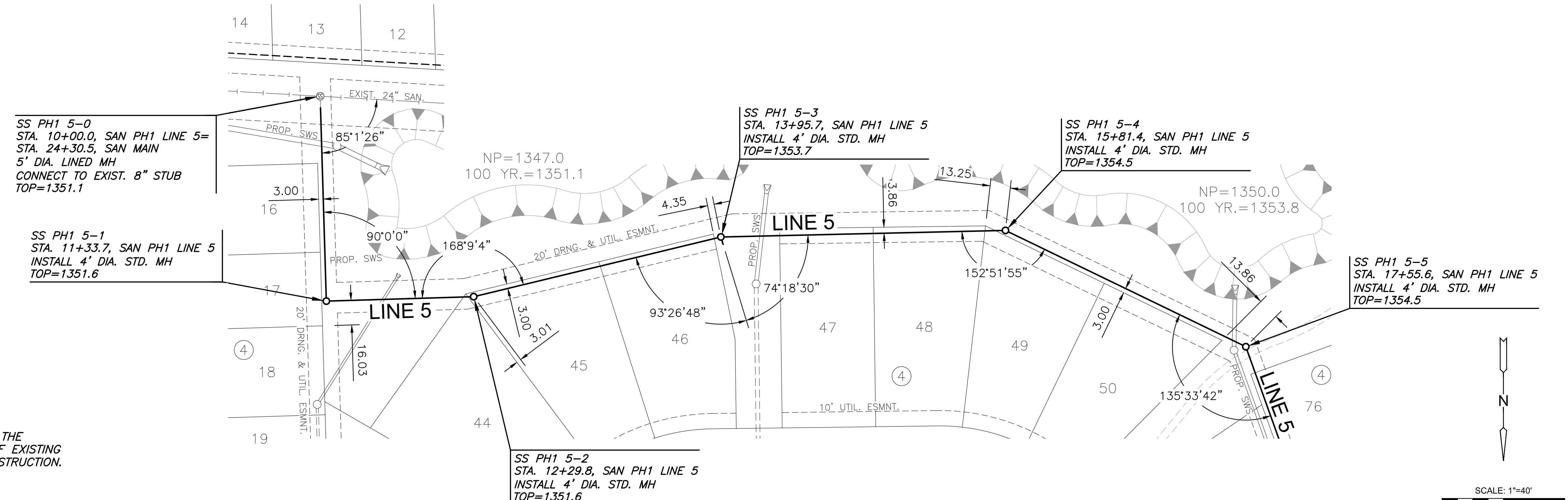
PLAN SAN PH1 LINE 5 PROFILE SAN PH1 LINE 5
