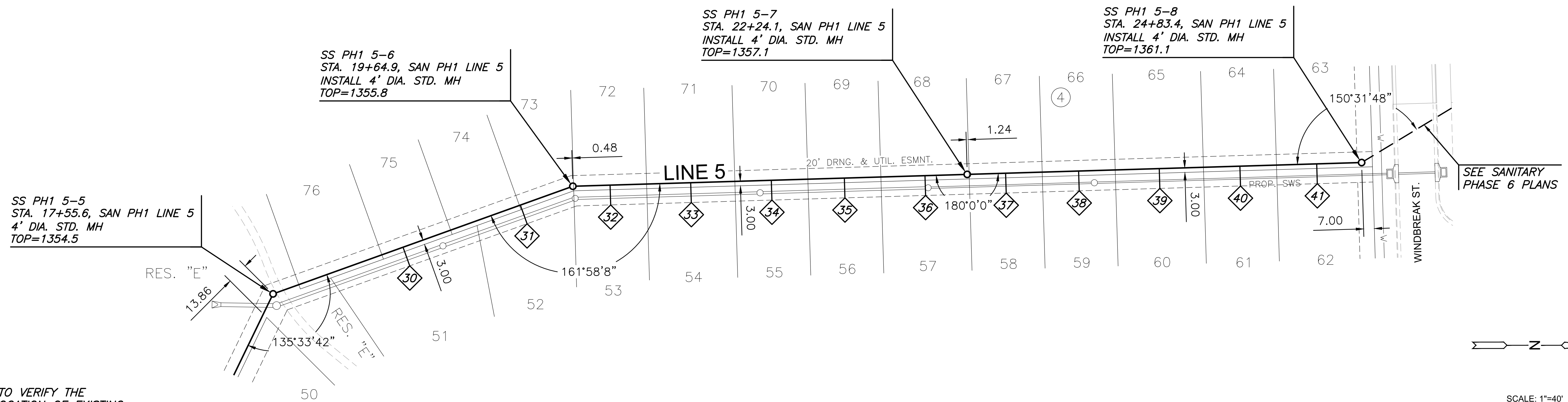
PLAN SAN PH1 LINE 5 (CONT.) PROFILE SAN PH1 LINE 5 (CONT.)
