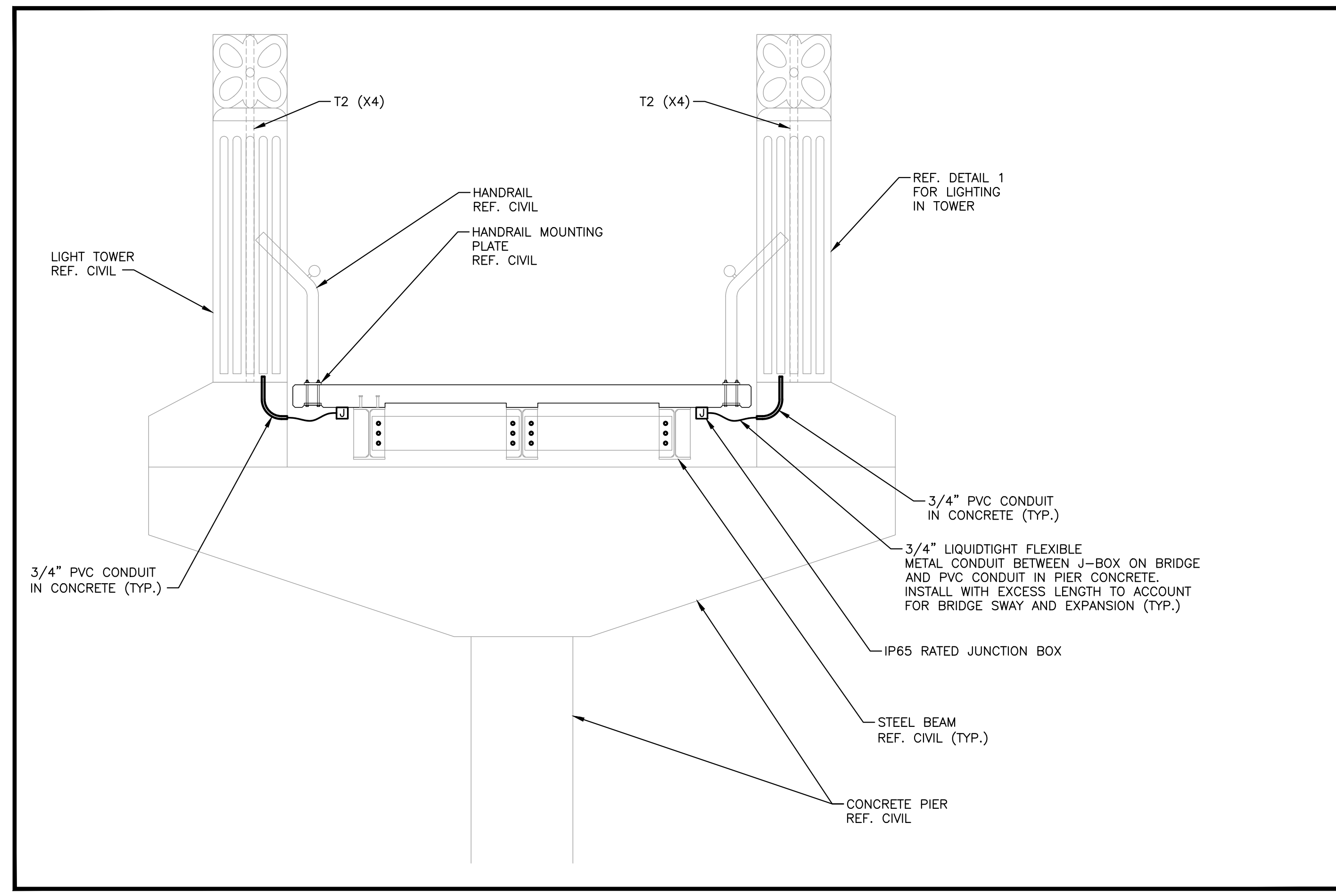
2 SLAB & PIER CONDUIT ROUTING DETAIL SCALE: 3/8"=1'-0"
