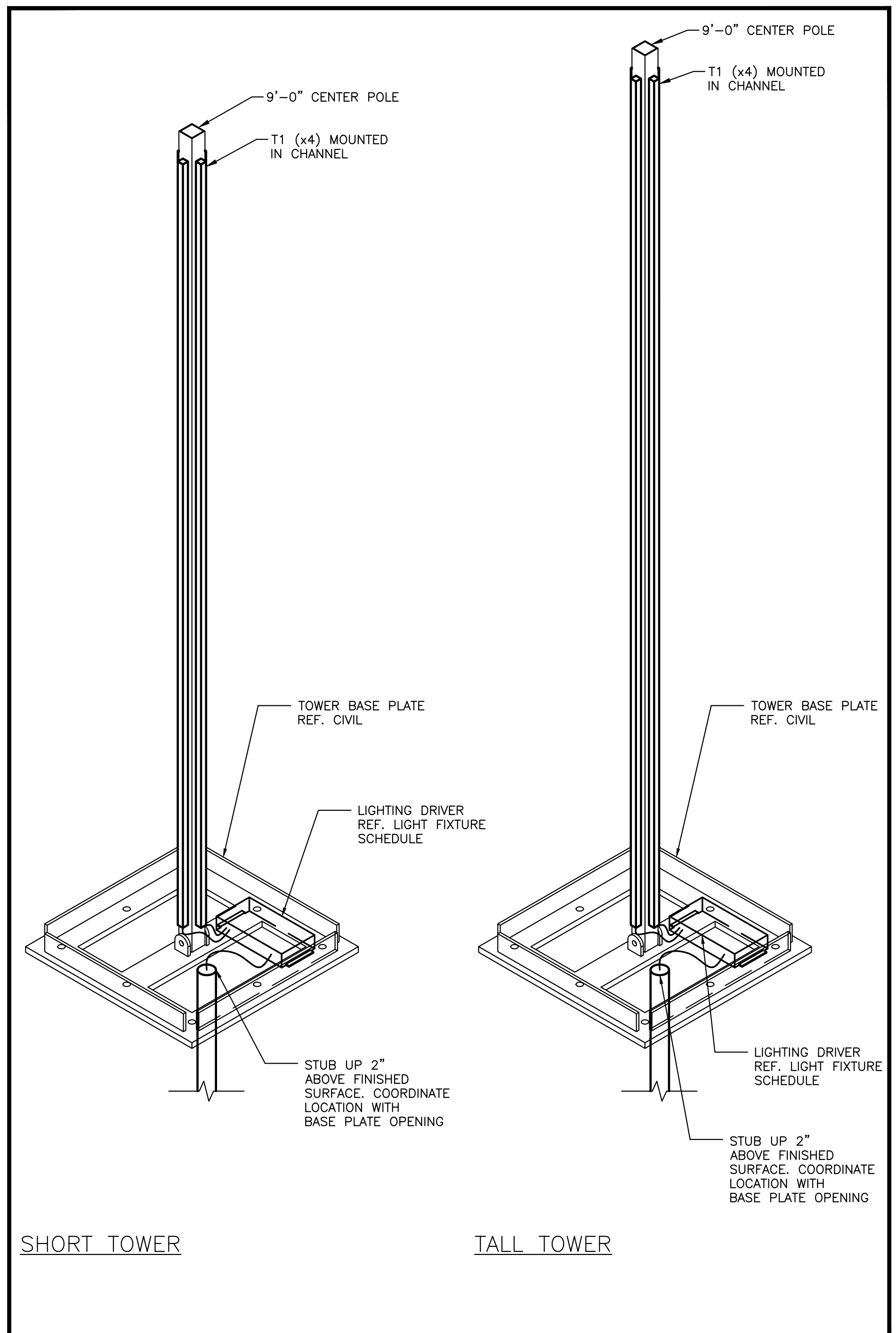
1 LIGHT TOWER DETAIL SCALE: 1"=1'-0"
